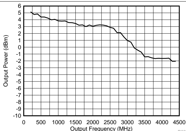
Figure 37. Power vs Output Frequency
