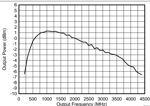
Figure 38. Power vs Output Frequency
