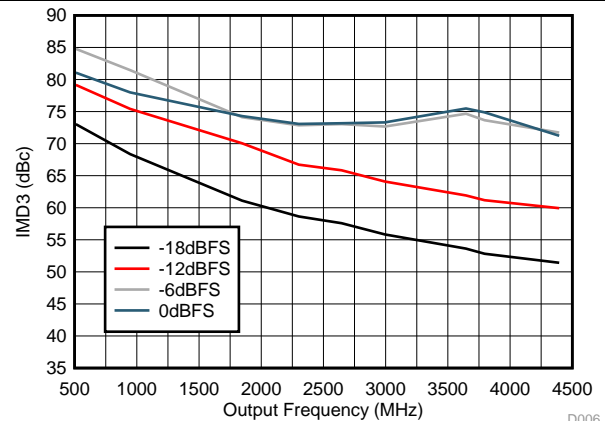
DAC38RF80/90/84
