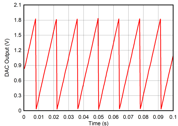
LED breathing effect in sawtooth pattern
