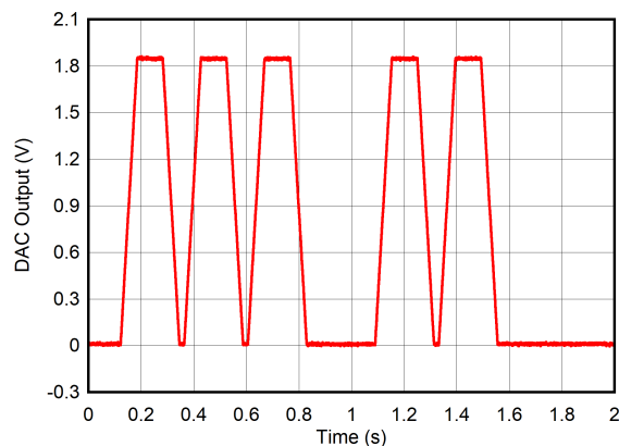
图 73. High-Priority Alarm
