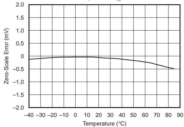
ZERO-SCALE ERROR vs TEMPERATURE (Code 0040 H )
