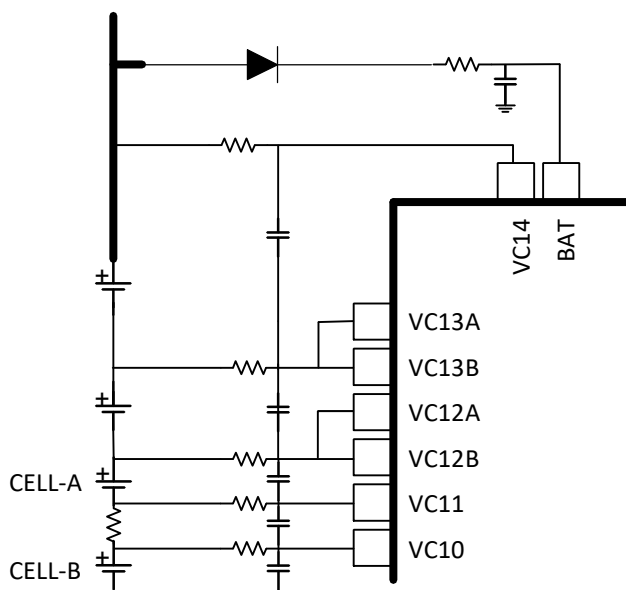
图 10-1. Using Cell Input Pins for Interconnect Measurement
