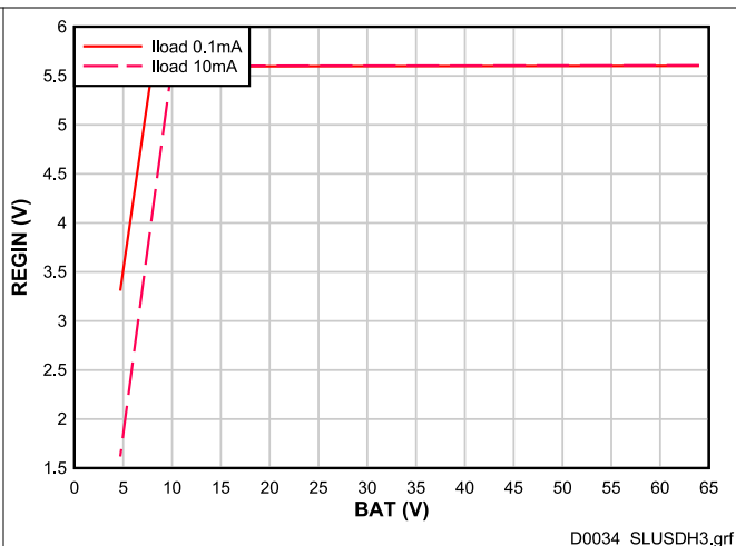
图 7-27. REGIN Voltage vs. BAT Voltage
