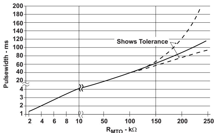
Figure 5. Relationship Between Trickle Pulse-Width and Value of R_{MTO}
