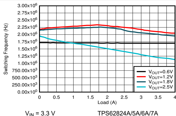
图 9-25. Switching Frequency
