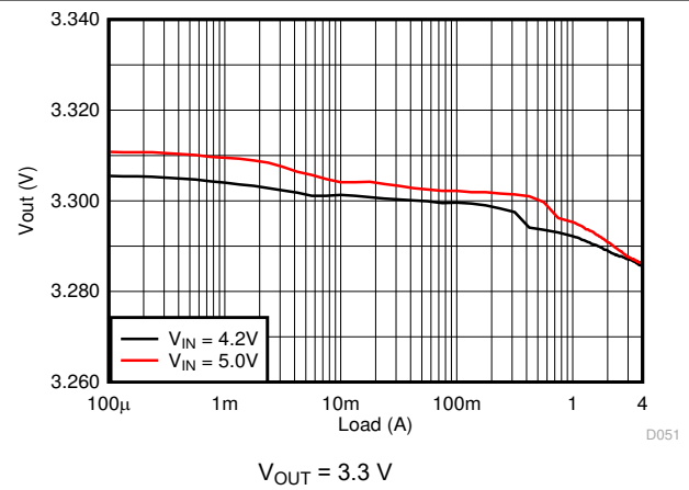
图 9-20. Load Regulation
