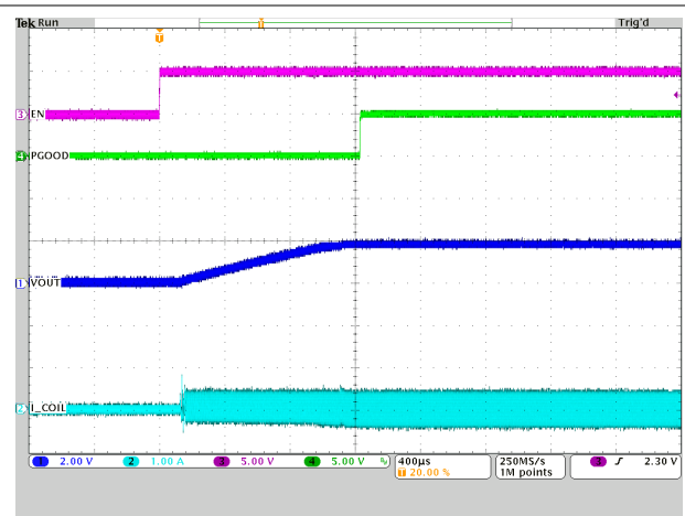
图 9-40. Start-up with No Load
