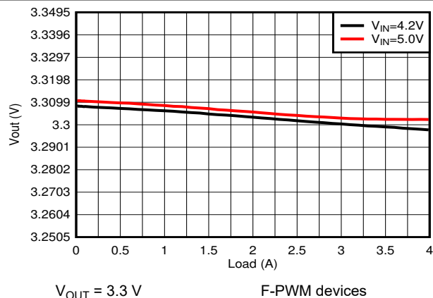
图 9-22. Load Regulation
