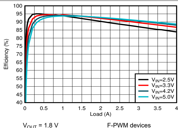
图 9-13. PWM Efficiency
