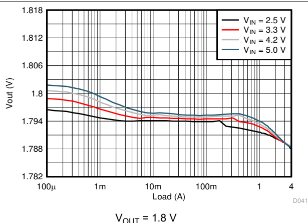
图 9-12. Load Regulation
