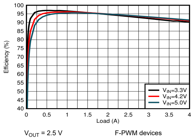
图 9-17. PWM Efficiency
