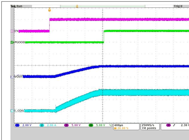
图 9-39. Start-up with Load
