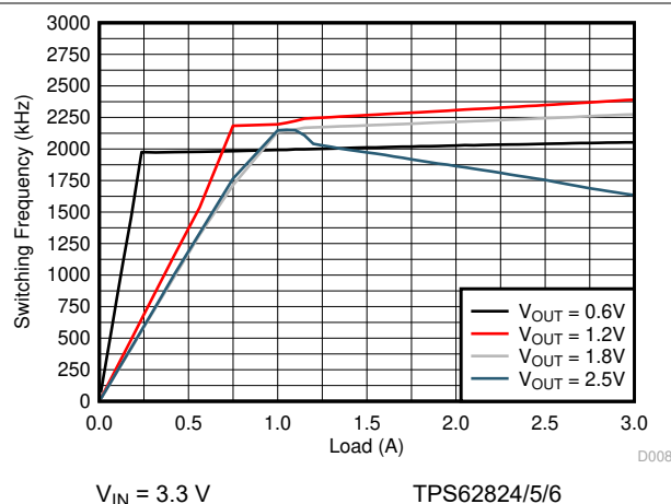
图 9-23. Switching Frequency
