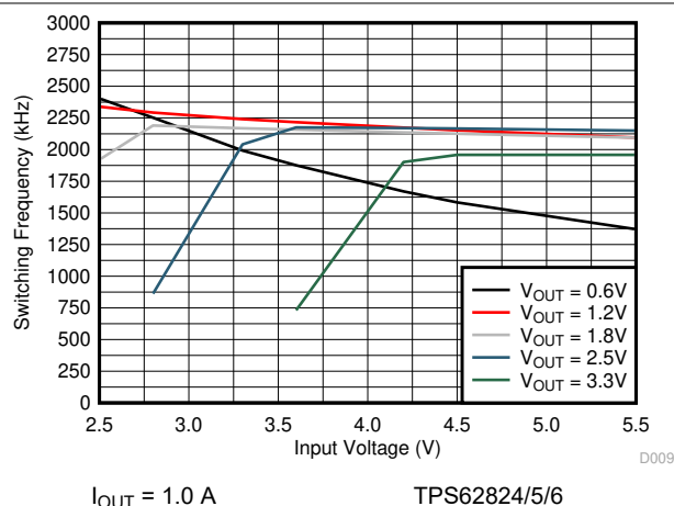
图 9-24. Switching Frequency
