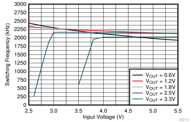
图 9-28. Switching Frequency
