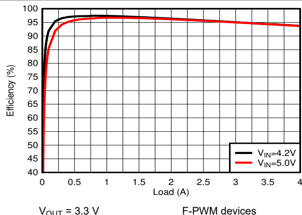
图 9-21. PWM Efficiency
