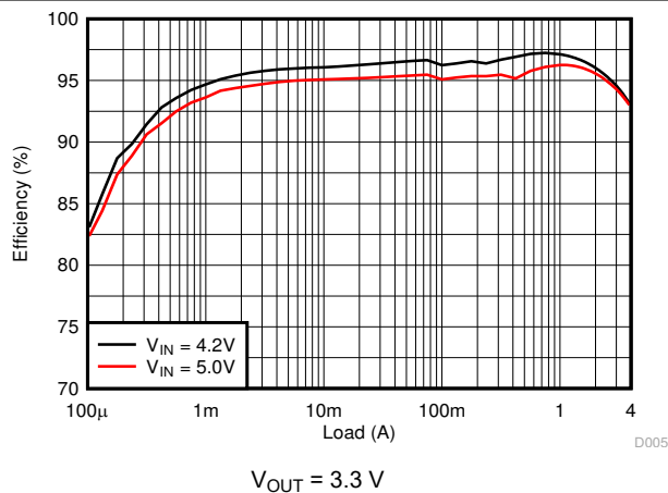
图 9-19. Efficiency
