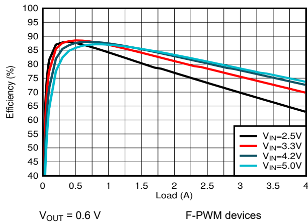
图 9-5. PWM Efficiency
