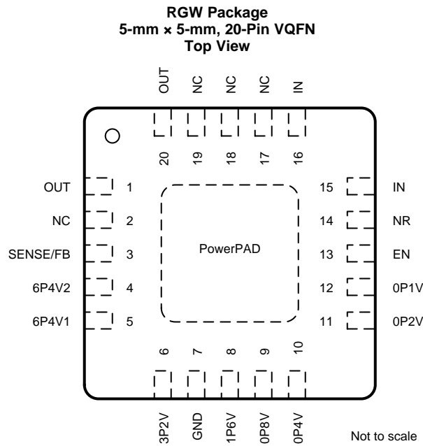
Pin Functions
