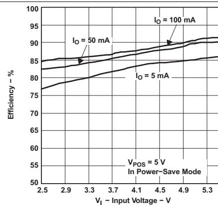
Figure 21. TPS65130 Efficiency vs Input Voltage
