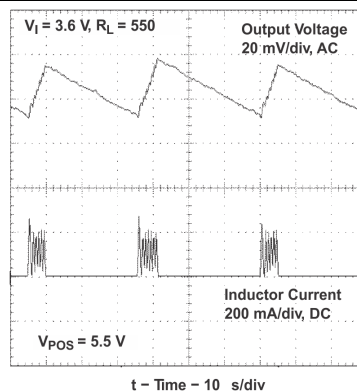
Figure 46. V_{POS} in Power-Save Mode
