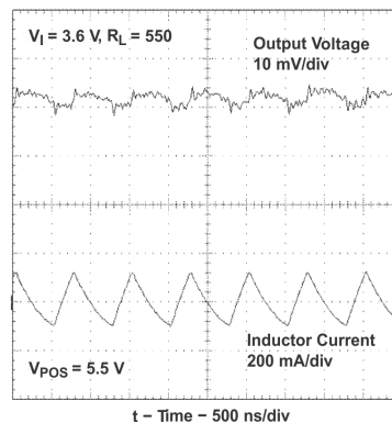
Figure 44. V_{POS} at Power-Save Mode Disabled
