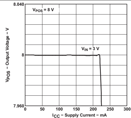
Figure 32. TPS65130 Output Voltage vs Output Current
