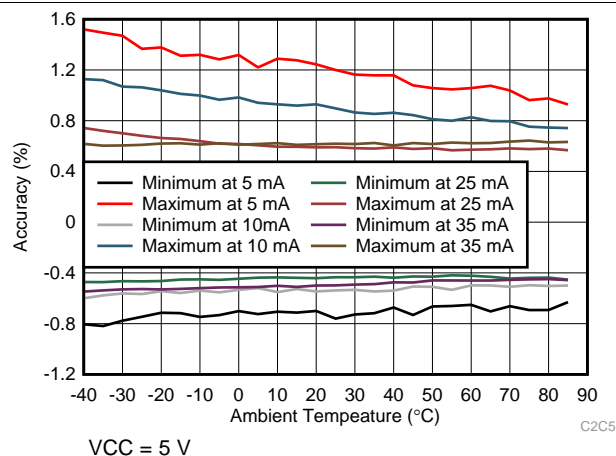
图 6. Channel-to-Channel Current Accuracy vs Temperature
