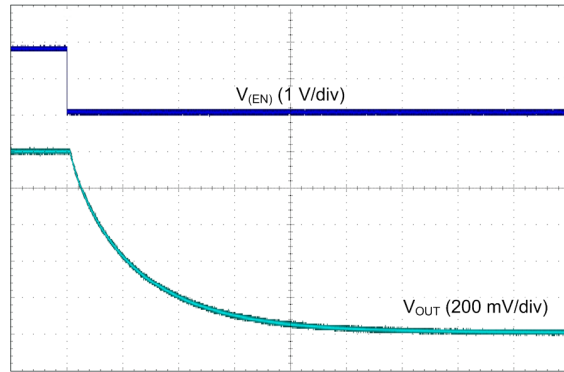
图 50. LDO Shutdown
