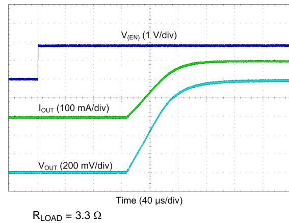
图 49. LDO Start-Up
