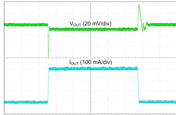
图 51. LDO Transient Load Step Response
