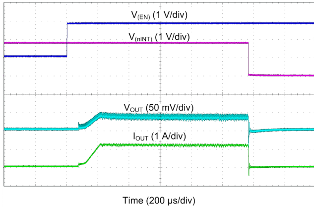
图 44. Buck Start-up With Short on Output
