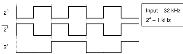
图 10. Application timing diagram
