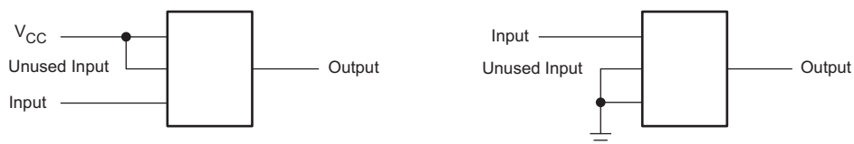
Figure 5. Layout Schematic
