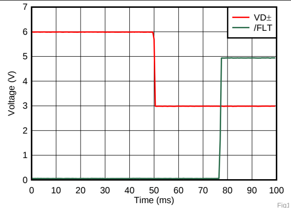
图 15. \overline{\text{FLT}} Recover Time After OVP Clear
