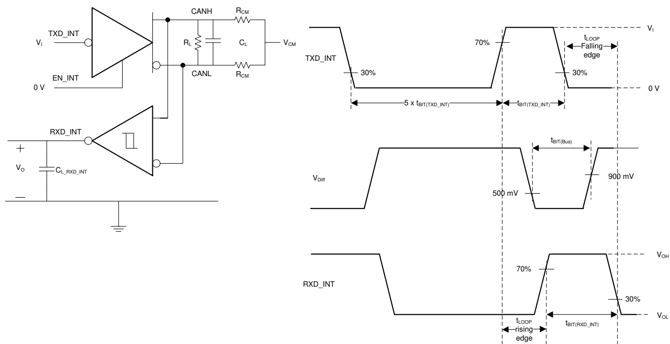
图 8. Transmitter and Receiver Timing Behavior Test Circuit and Measurement
