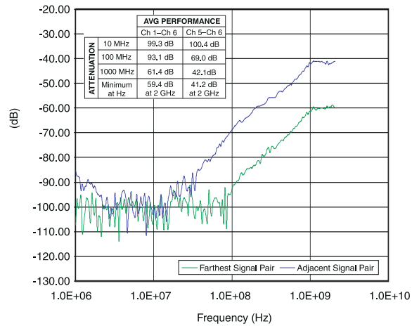
Figure 6-1. Channel-to-Channel Crosstalk
