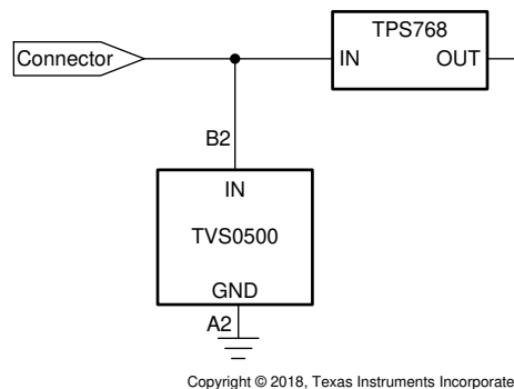
图 10. TVS0500 Application Schematic
