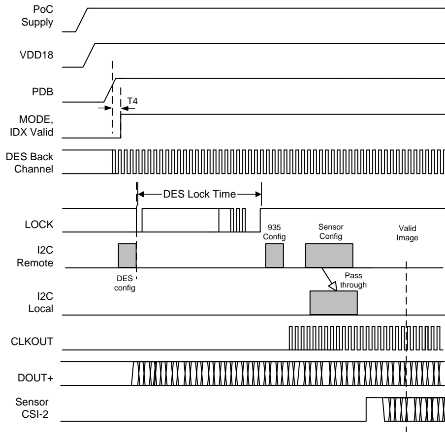
图 23. Initialization Sequence: Synchronous Cloning Mode
