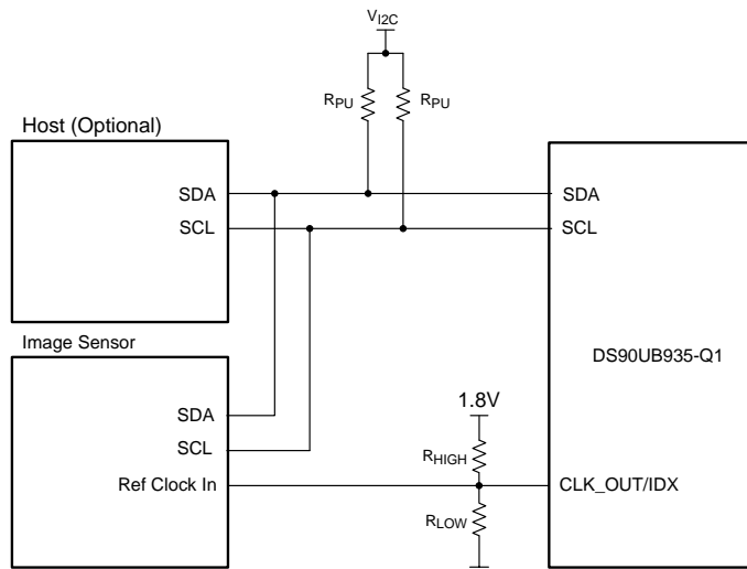
图 11. Circuit to Bias IDX Pin
