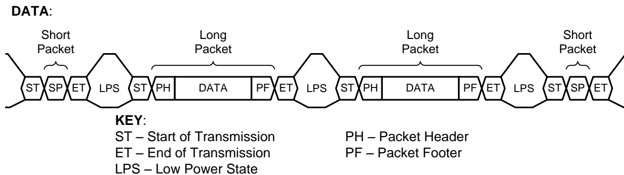
图 4. CSI-2 Protocol Layer With Short and Long Packets
