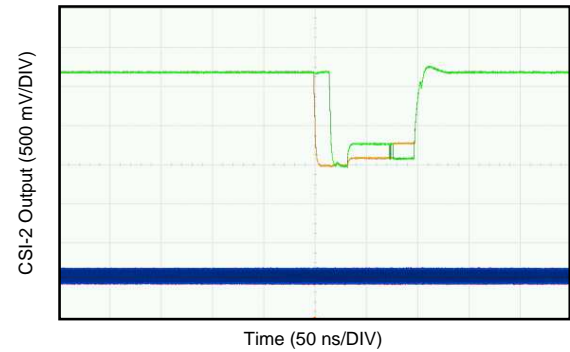
Figure 42. CSI-2 DATA and Continuous CLK Output
