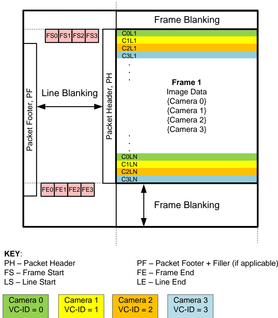
Figure 30. Basic Synchronized Format
