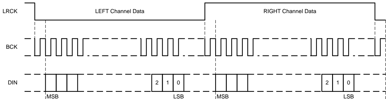
Figure 16. Stereo I²S Format
