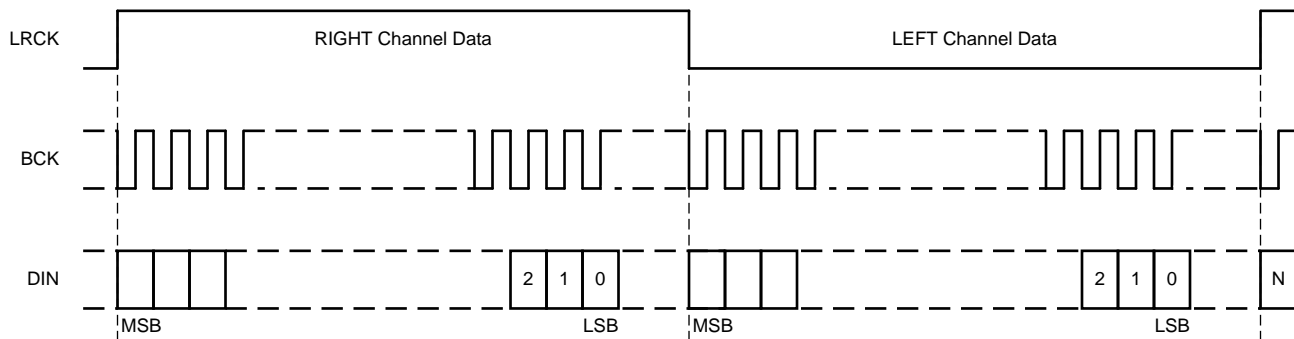
Figure 17. Left-Justified Format
