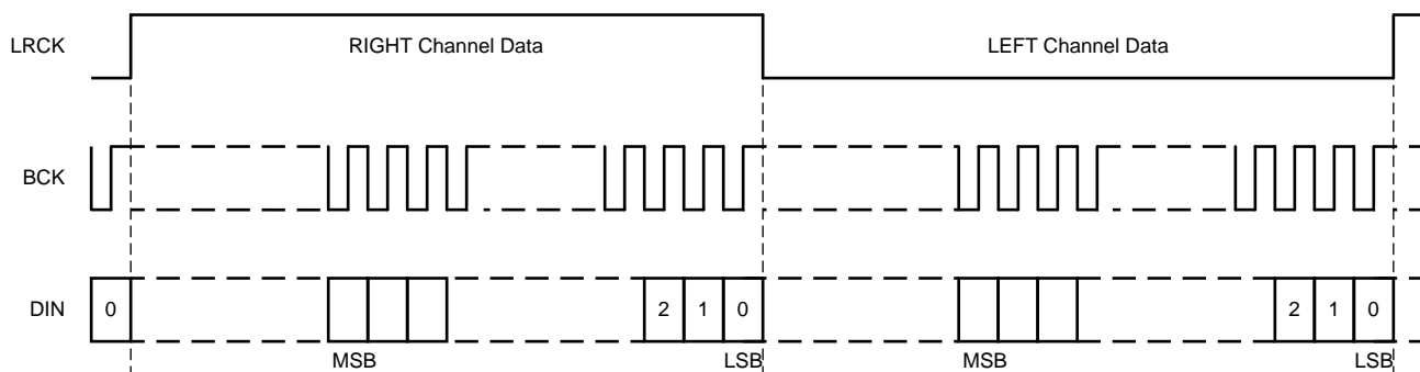
Figure 18. Right-Justified Format
