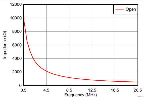
Figure 8. Input Impedance Magnitude vs Frequency
