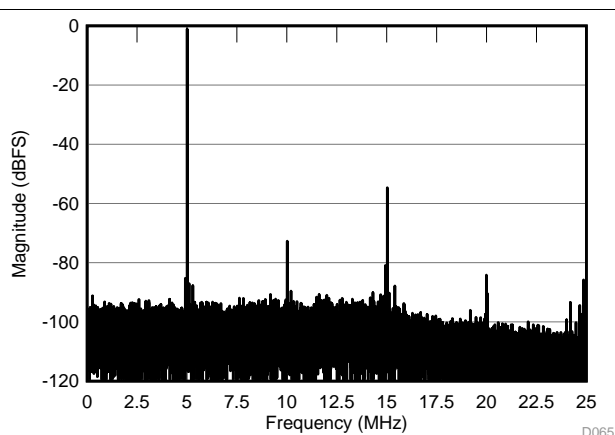
Figure 106. FFT for VCNTL = 0.9 V
