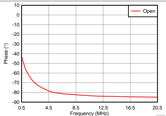
Figure 9. Input Impedance Phase vs Frequency
