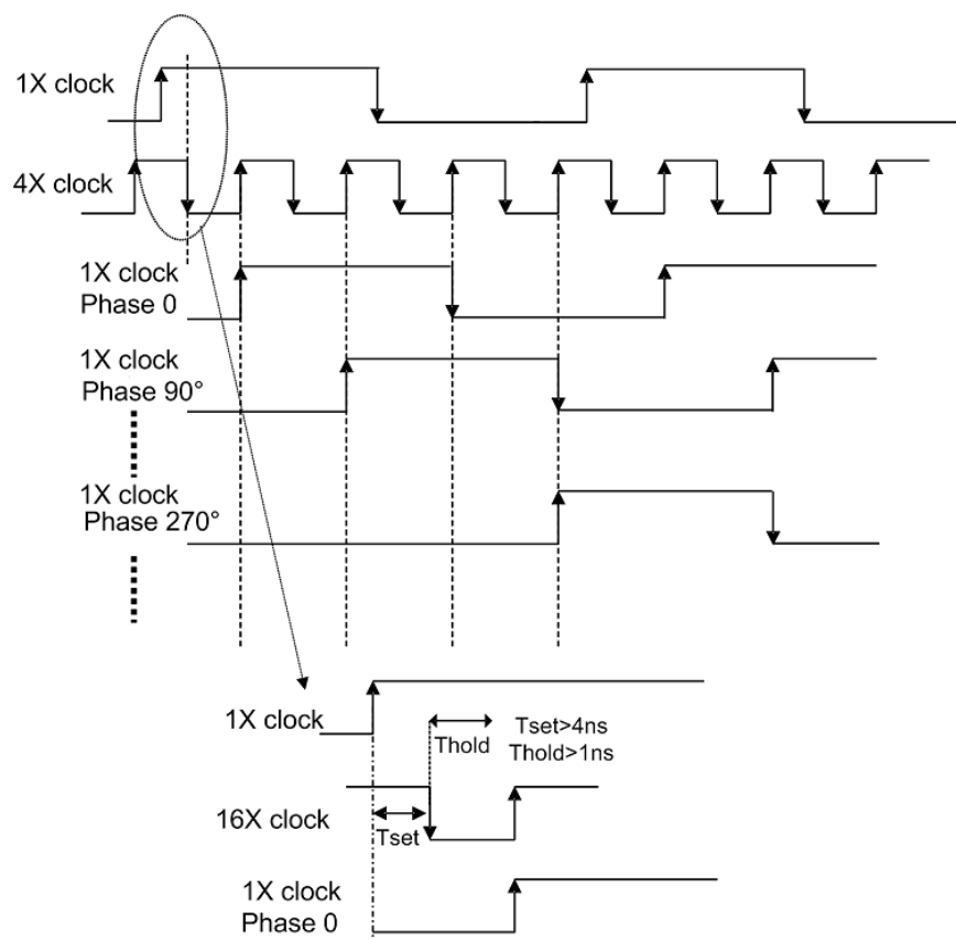
Figure 92. 8 \times f_{cw} and 4 \times f_{cw} Timing Diagram
