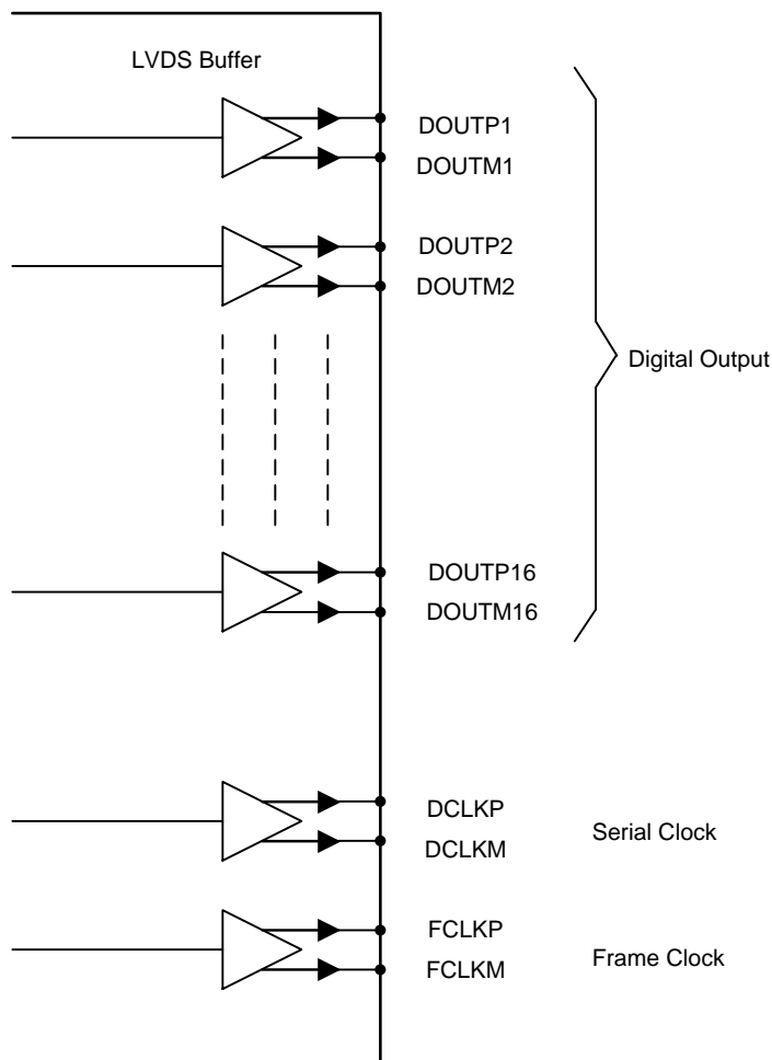
Figure 75. LVDS Output
