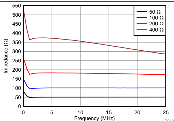
Figure 8. Input Impedance Magnitude vs Frequency
