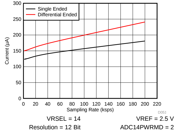
图 5-31. Current vs Sampling Rate
