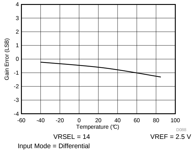
图 5-68. Gain Error vs Temperature
