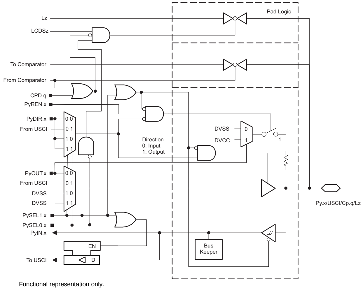
图 6-15. Py.x/USCI/Cp.q Port Schematic
