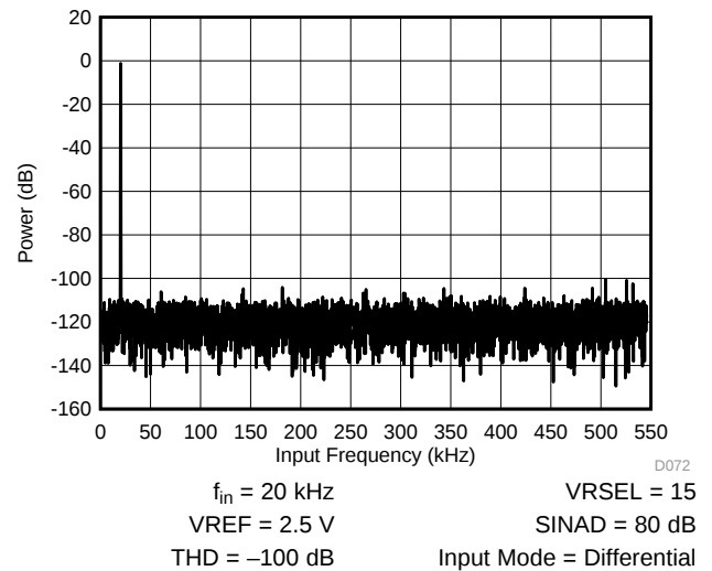
图 5-52. Power vs Input Frequency
