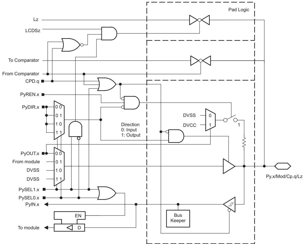
图 6-18. Py.x/Mod/Cp.q/Lz Port Schematic
