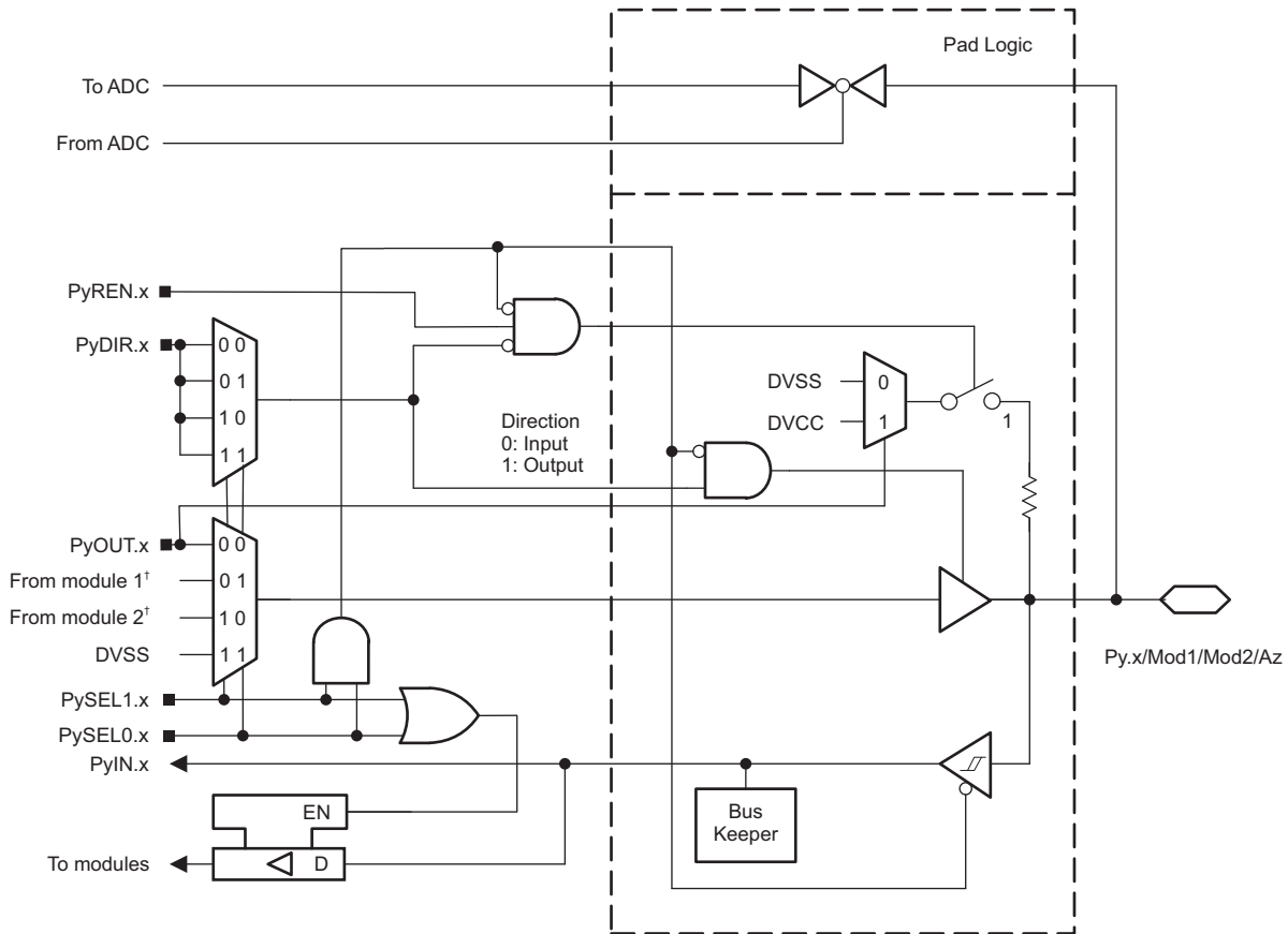
图 6-12. Py.x/Mod1/Mod2/Az Port Schematic
