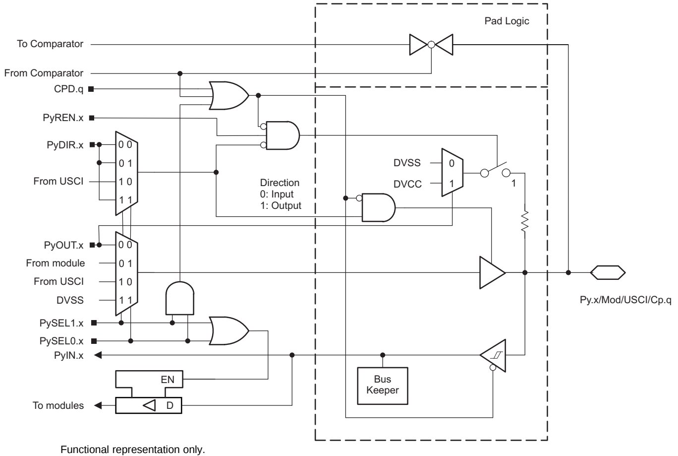
图 6-16. Py.x/Mod/USCI/Cp.q Port Schematic
