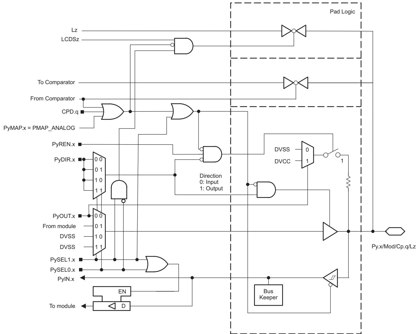
图 6-19. Py.x/Mod/Cp.q/Lz Port Schematic
