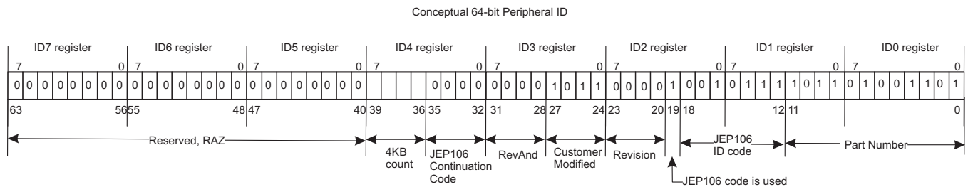
图 6-25. ROM PID Entries for MSP432P4x1x Device
