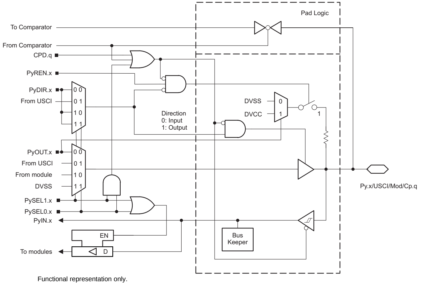
图 6-17. Py.x/USCI/Mod/Cp.q Port Schematic
