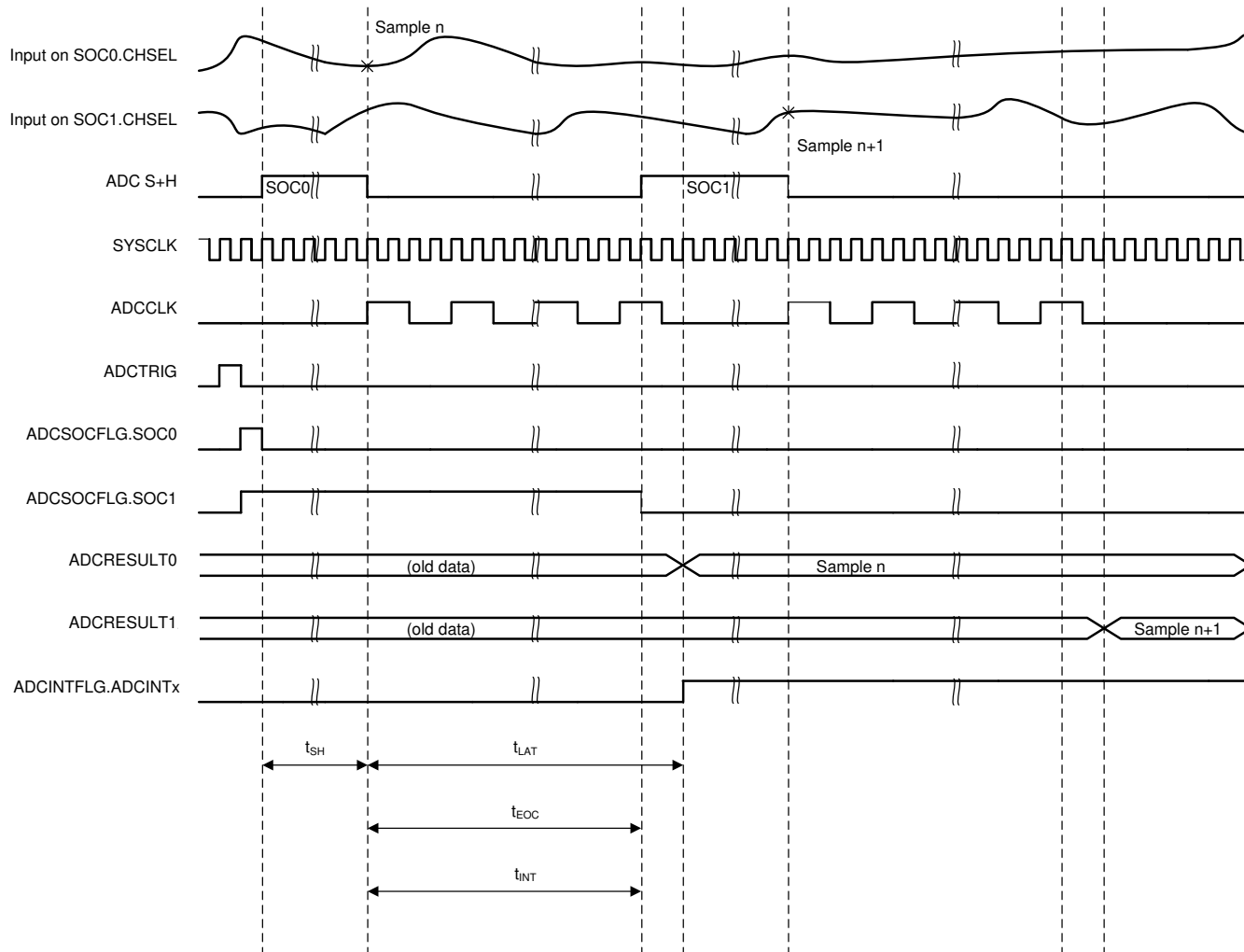
图 7-35. ADC Timings
