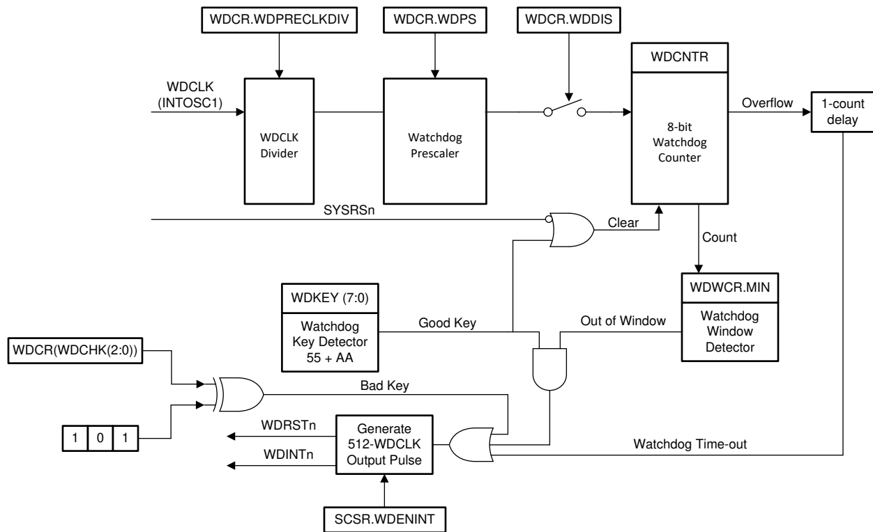
图 8-3. Windowed Watchdog
