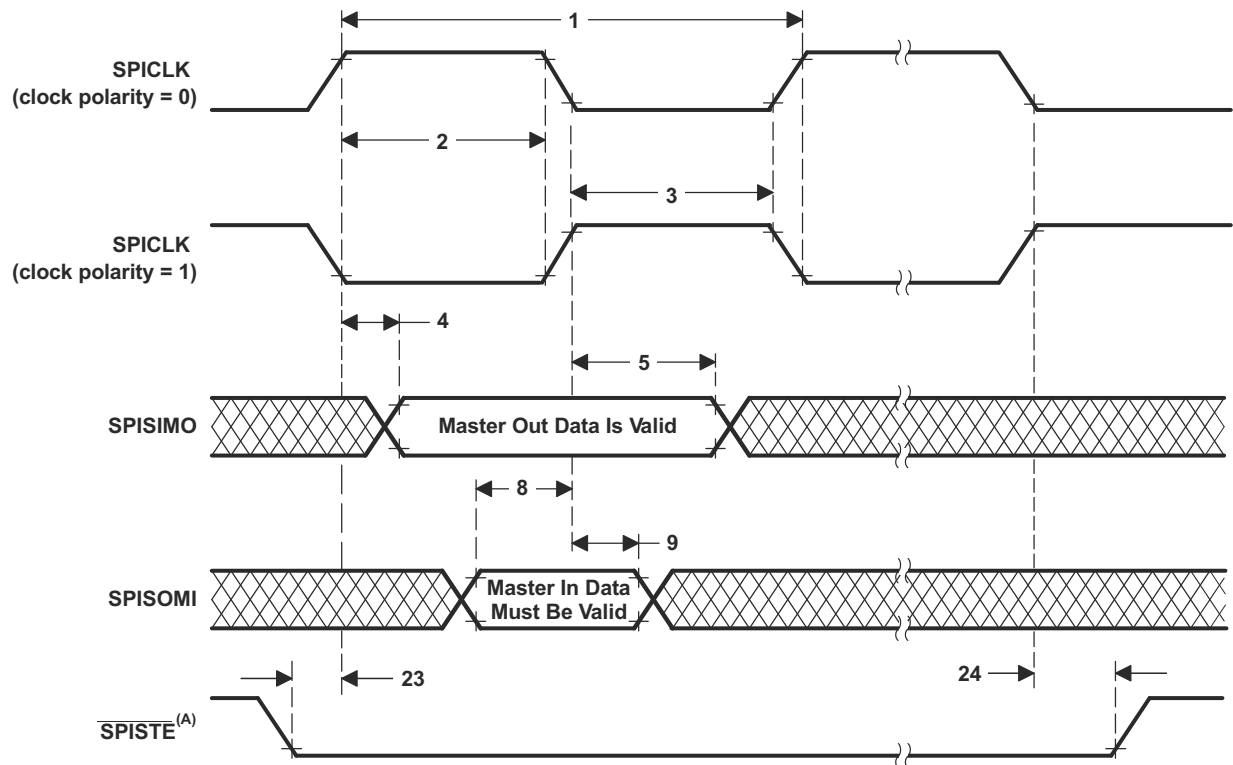
图 7-58. SPI Master Mode External Timing (Clock Phase = 0)
