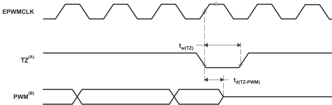
图 7-45. PWM Hi-Z Characteristics
