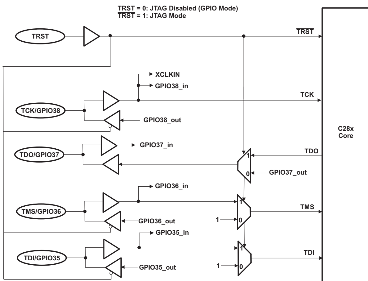
Figure 6-44. JTAG/GPIO Multiplexing
