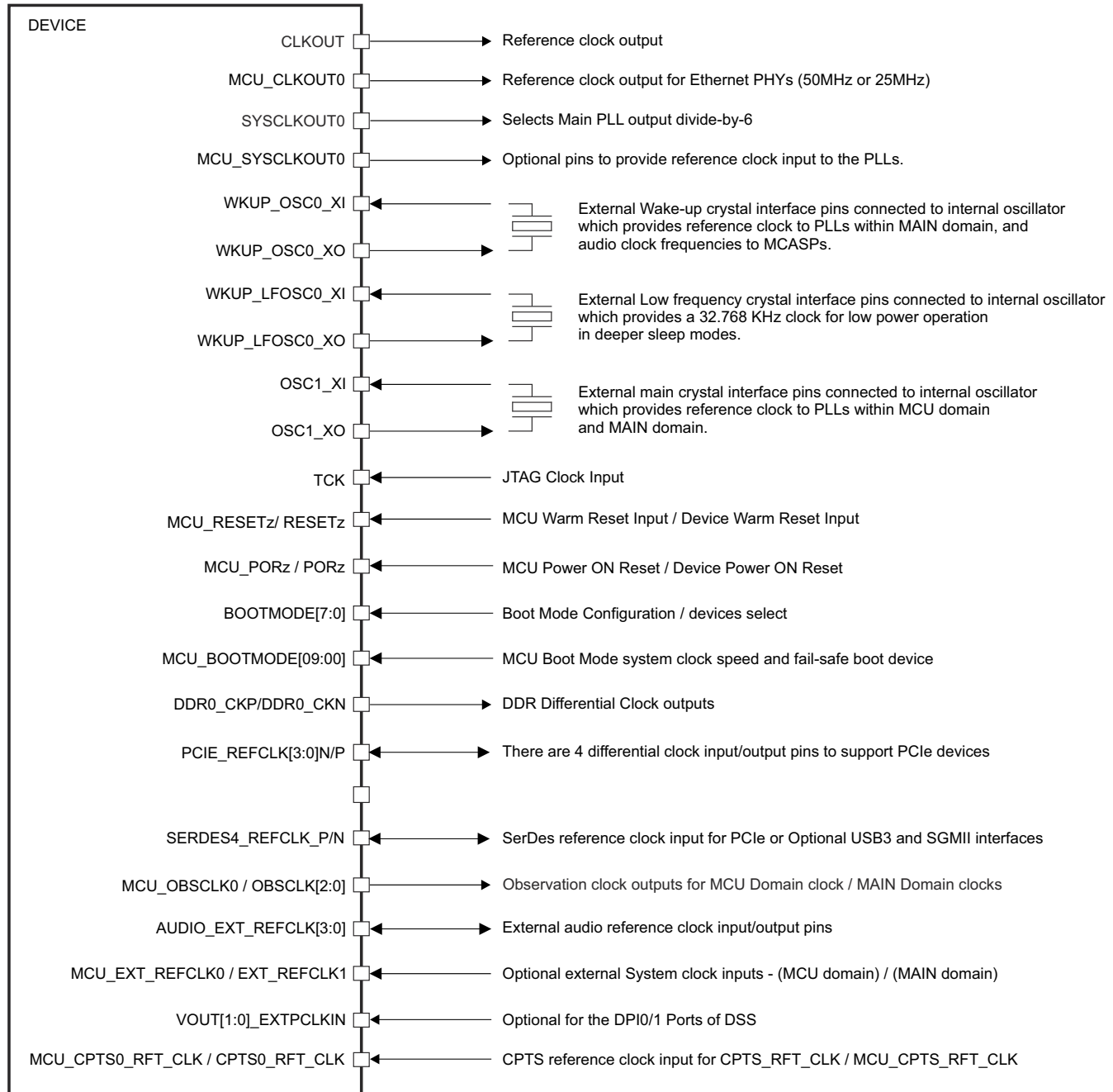
Figure 7-22. Input Clocks Interface
