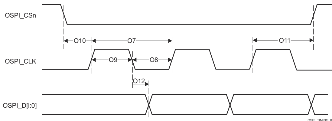
Figure 7-109. OSPI Switching Characteristics – SDR
