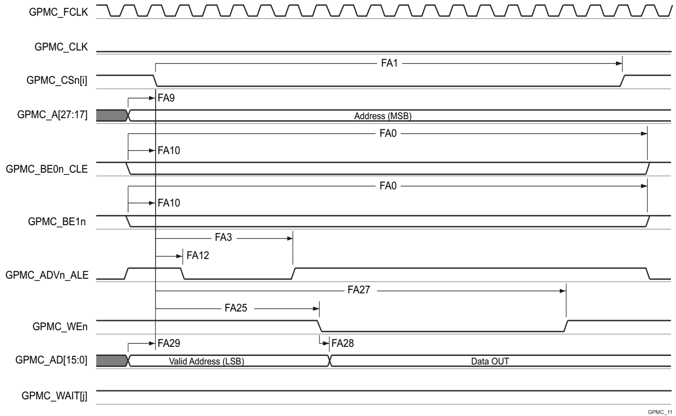
Figure 7-72. GPMC and Multiplexed NOR Flash — Asynchronous Write — Single Word
