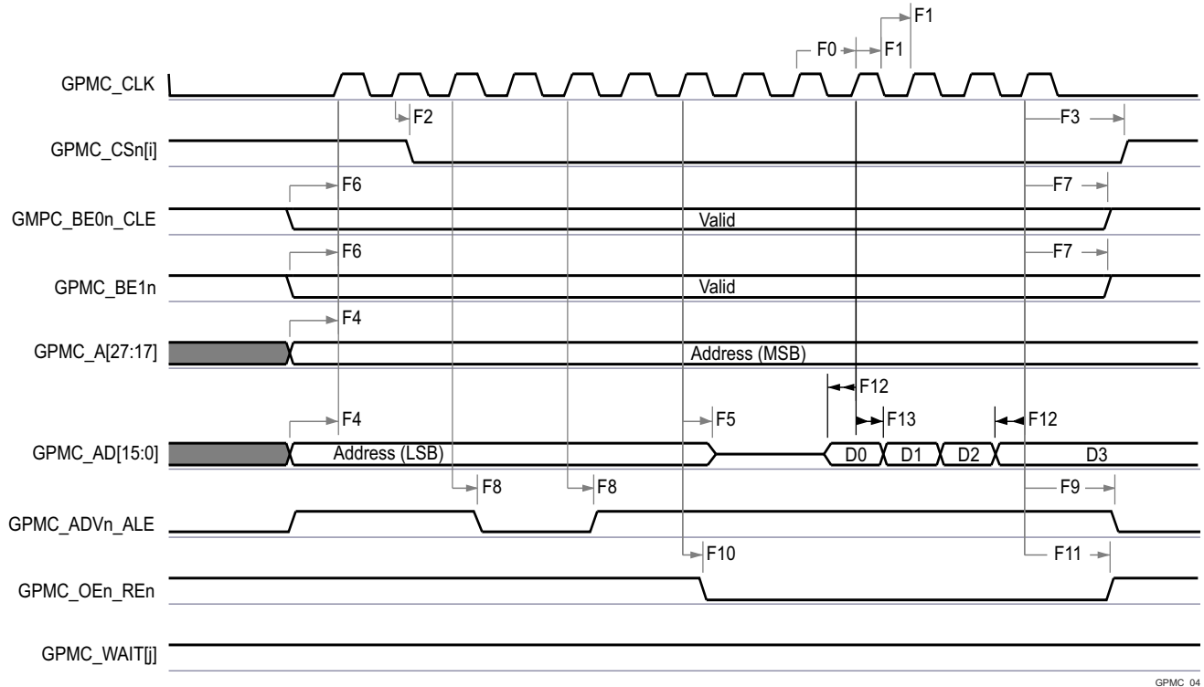
Figure 7-64. GPMC and NOR Flash—Synchronous Burst Write (GPMCFCLKDIVIDER = 0)
