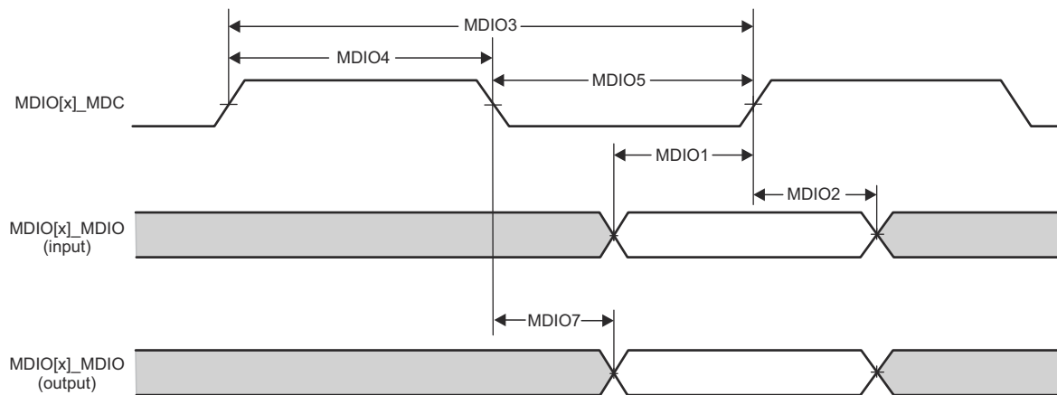
Figure 7-46. CPSW9G MDIO Diagrams Receive and Transmit
