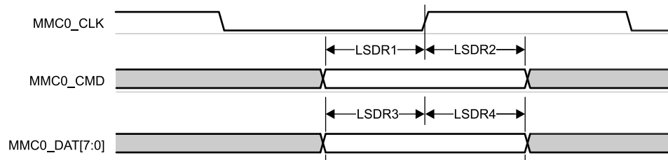
Figure 7-89. MMC0 – Legacy SDR – Receive Mode
