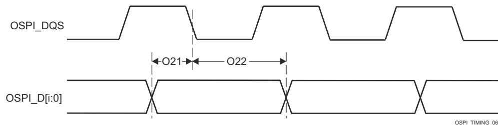
Figure 7-113. OSPI Timing Requirements – SDR, External Loopback Clock
