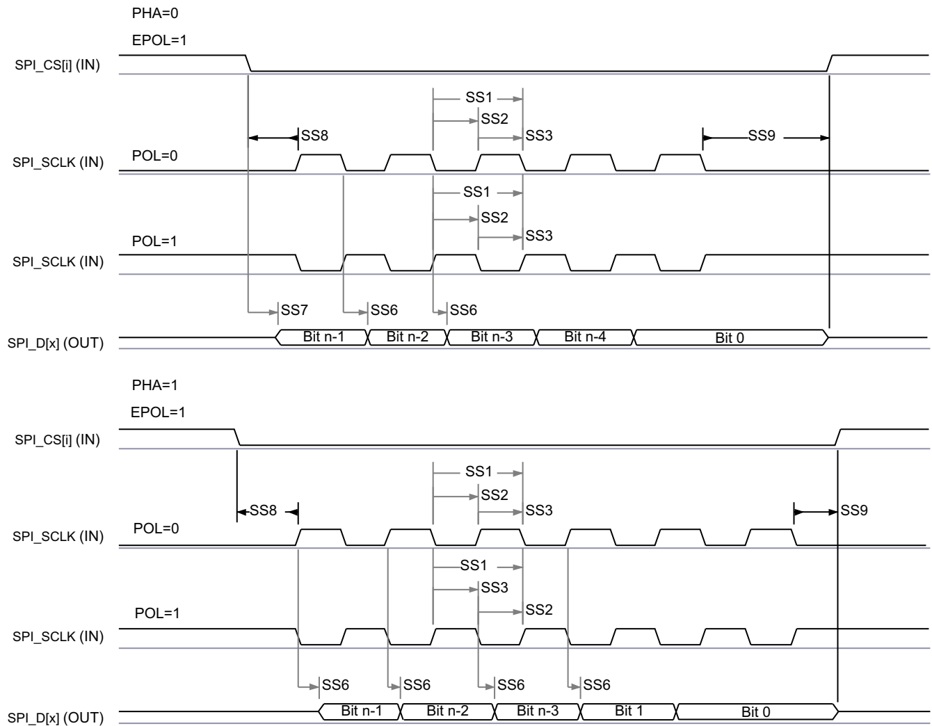
Figure 7-88. MCSPI Slave Mode Transmit Timing
