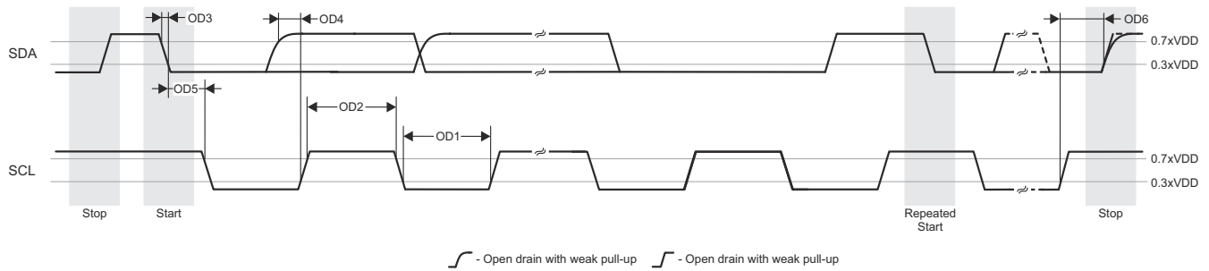
Figure 7-80. I3C Open Drain Timing Requirements
