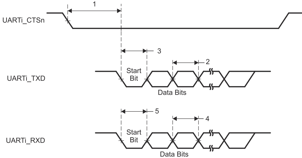
Figure 7-118. UART Timing
