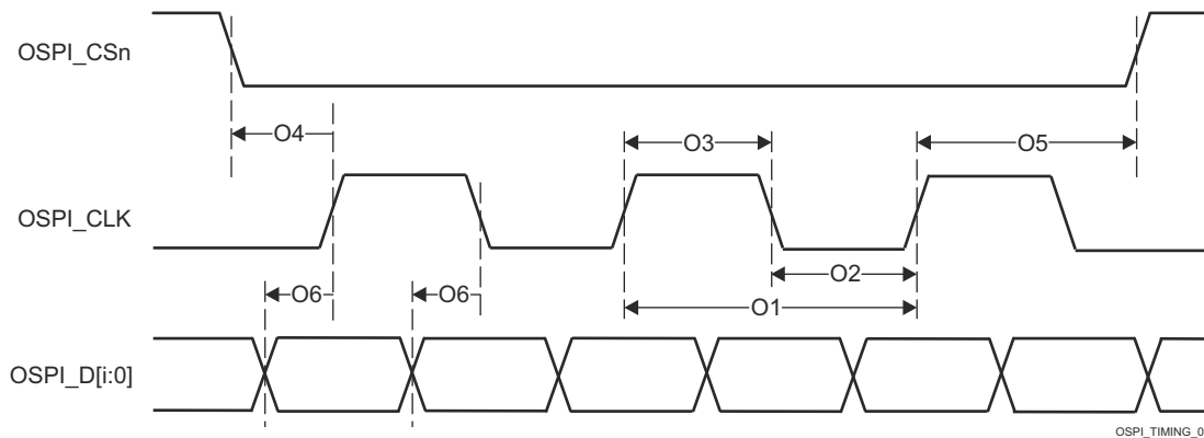
Figure 7-108. OSPI Switching Characteristics – DDR
