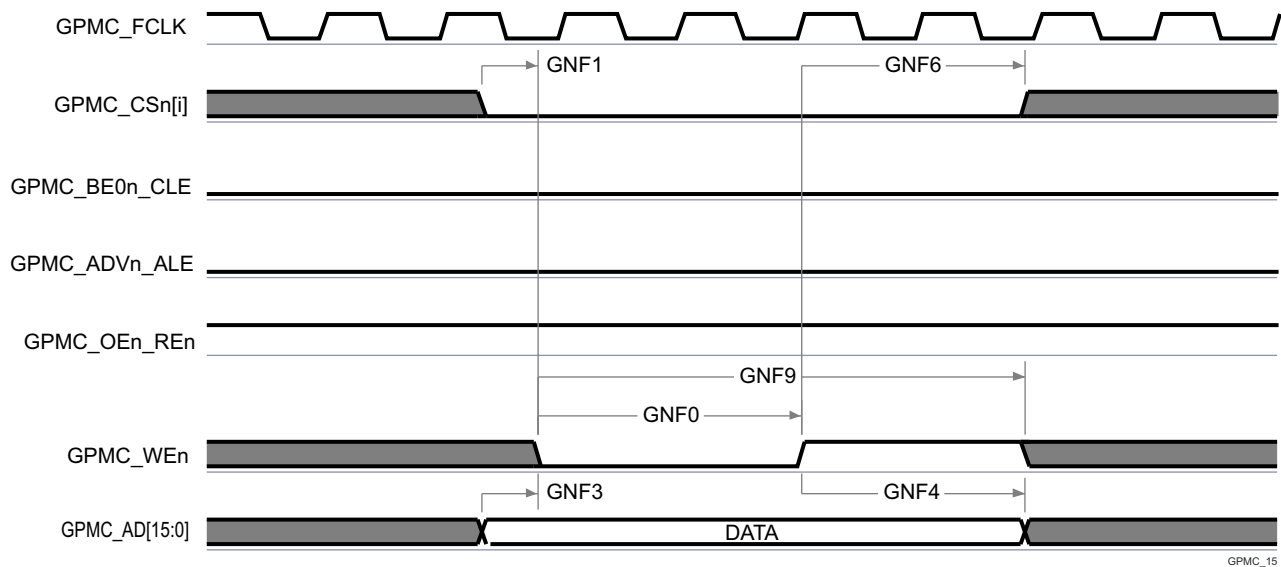
Figure 7-76. GPMC and NAND Flash — Data Write Cycle
