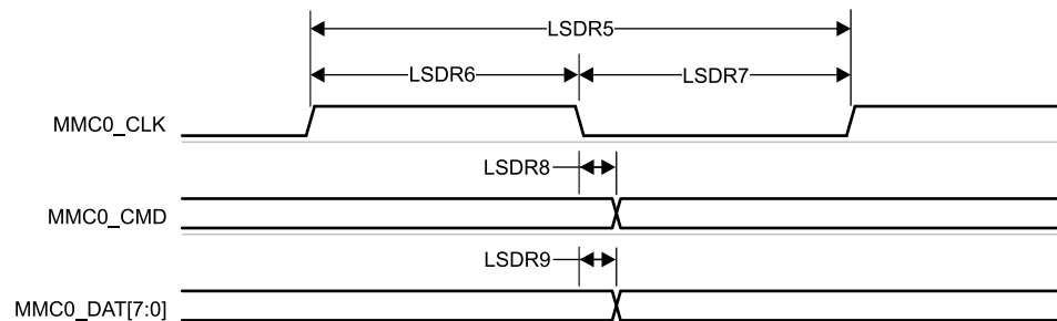
Figure 7-90. MMC0 – Legacy SDR – Transmit Mode
