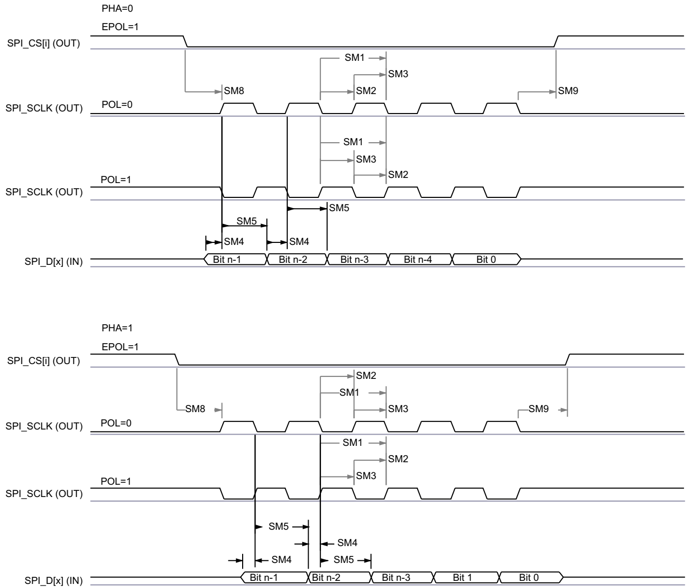
Figure 7-85. SPI Master Mode Receive Timing
