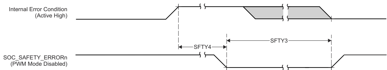
Figure 7-19. SOC_SAFETY_ERRORn Switching Characteristics
