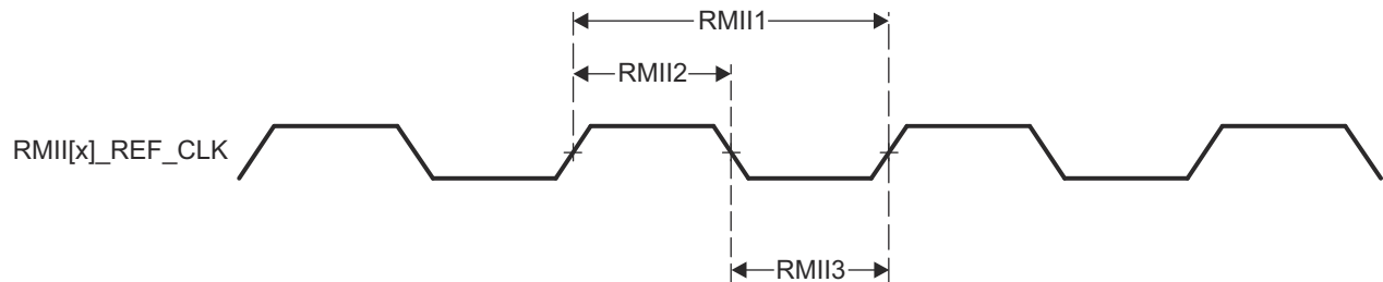
Figure 7-47. RMII[x]_REF_CLK Timing Requirements – RMII Mode
