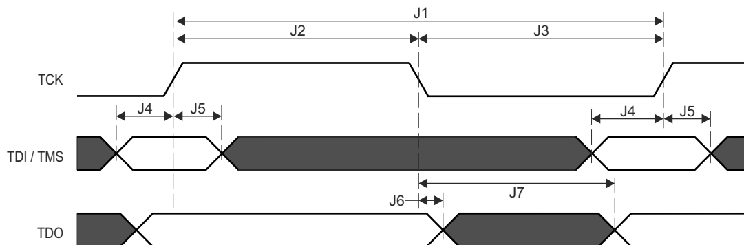
Figure 7-120. JTAG Timing Requirements and Switching Characteristics
