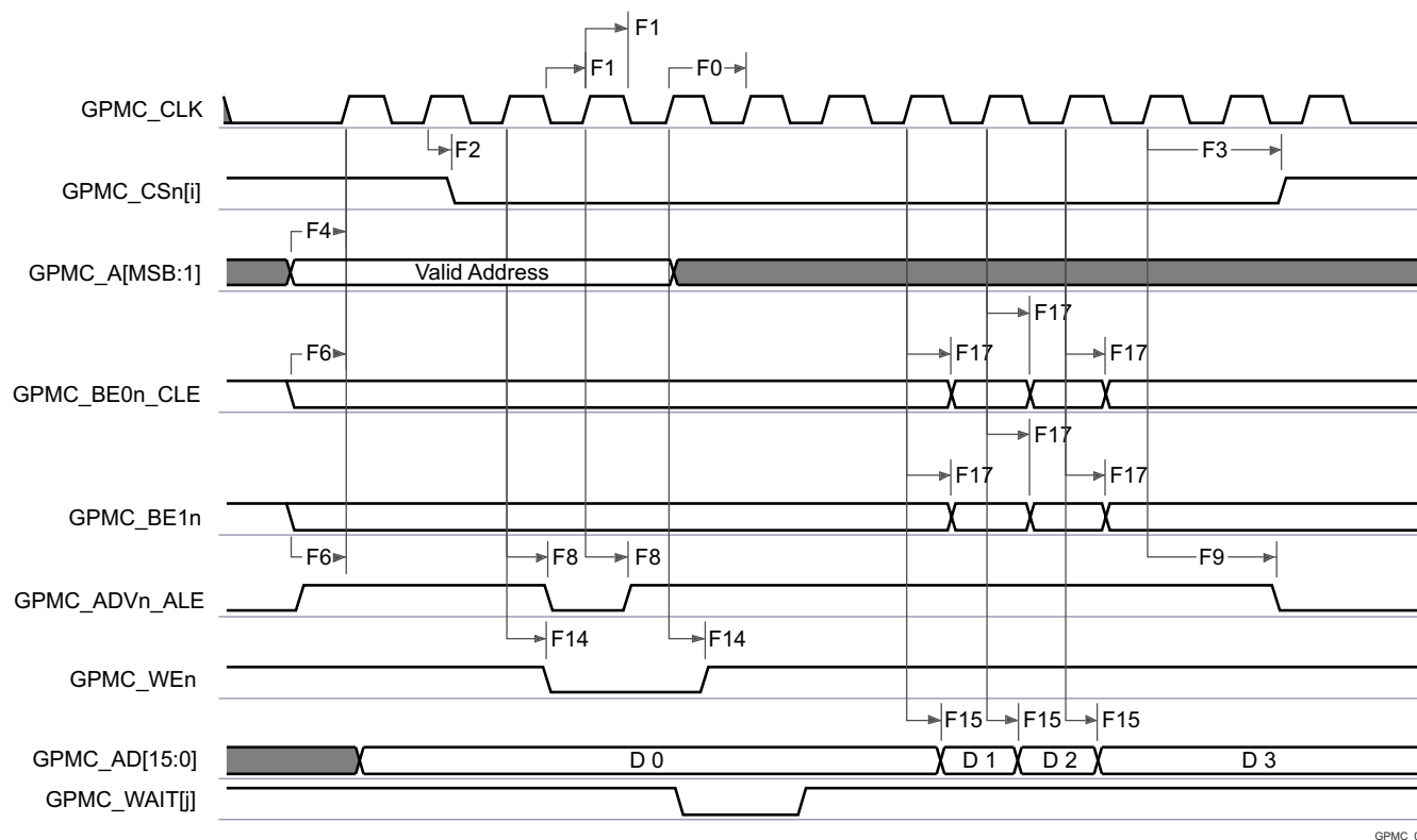
Figure 7-63. GPMC and NOR Flash — Synchronous Burst Read — 4x16-bit (GPMCCLKDIVIDER = 0)
