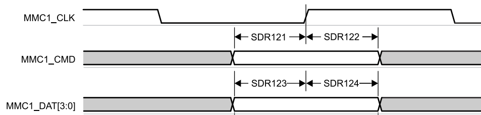
Figure 7-100. MMC1/2 – UHS-I SDR12 – Receive Mode
