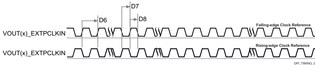
Figure 7-54. DPI External Pixel Clock Input
