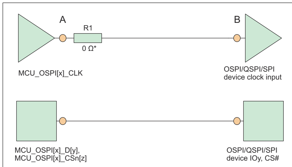
Figure 9-2. OSPI Interface High Level Schematic
