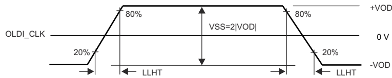
Figure 7-116. LVDS Output Transition Times
