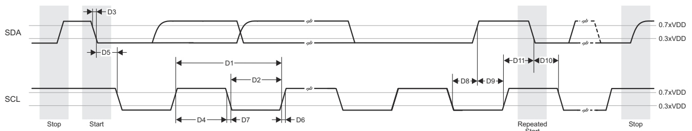
Figure 7-82. I3C Push-Pull Timing Requirements - SDR Mode
