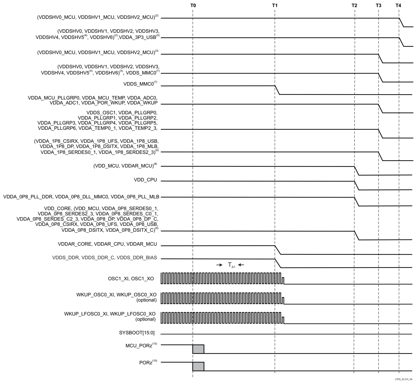
Figure 7-6. Independent MCU and Main Domains, Primary Power- Down Sequencing
