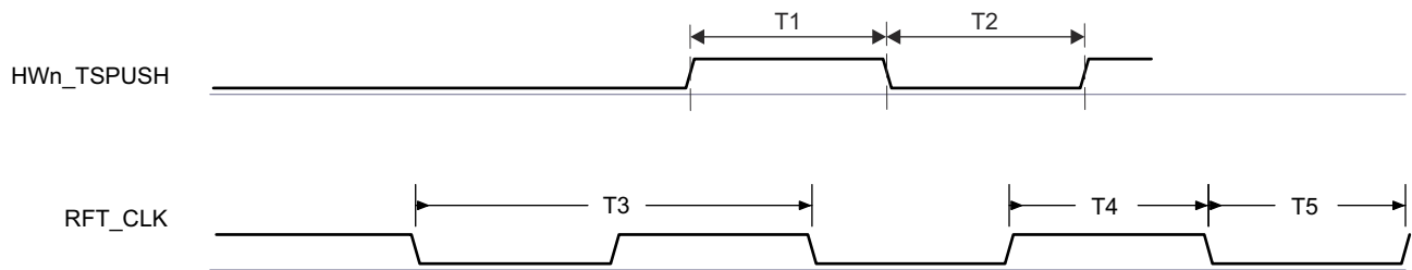
Figure 7-106. CPTS Timing Requirements
