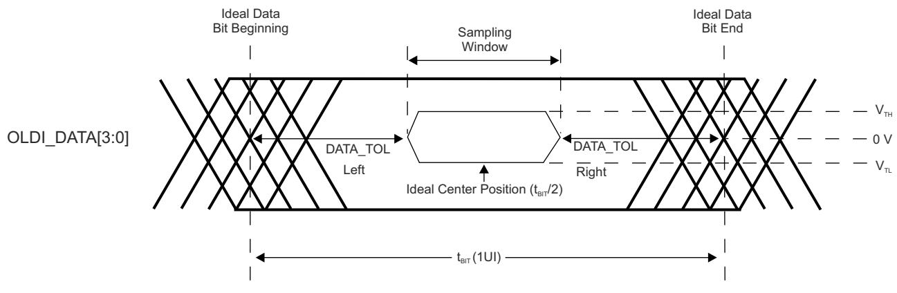
Figure 7-115. OLDI Data Output Jitter
