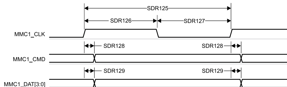
Figure 7-101. MMC1/2 – UHS-I SDR12 – Transmit Mode
