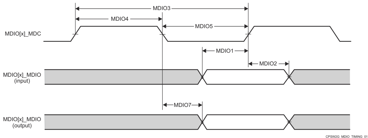
Figure 7-40. CPSW2G MDIO Timing Requirements and Switching Characteristics
