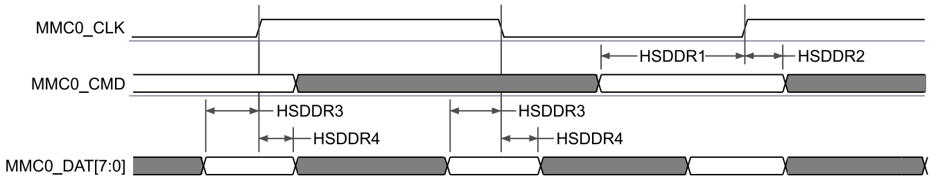
Figure 7-93. MMC0 – High Speed DDR Mode – Receive Mode
