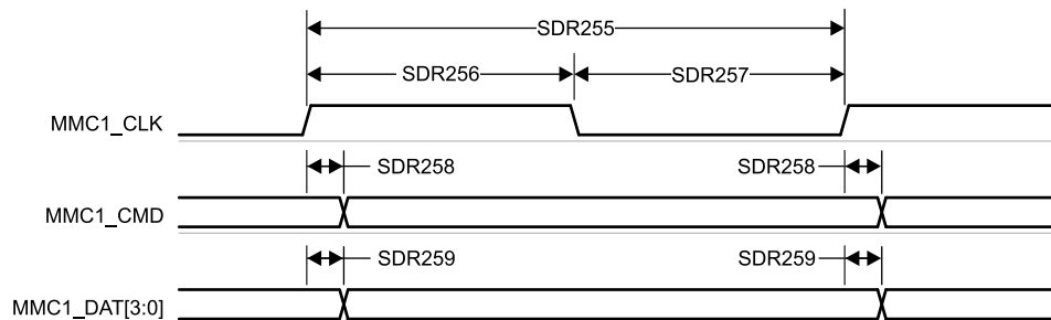
Figure 7-103. MMC1/2 – UHS-I SDR25 – Transmit Mode
