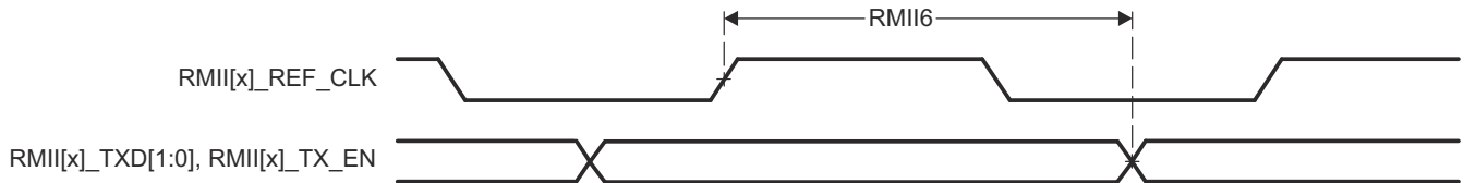
Figure 7-43. RMII[x]_TXD[1:0], and RMII[x]_TX_EN Switching Characteristics – RMII Mode
