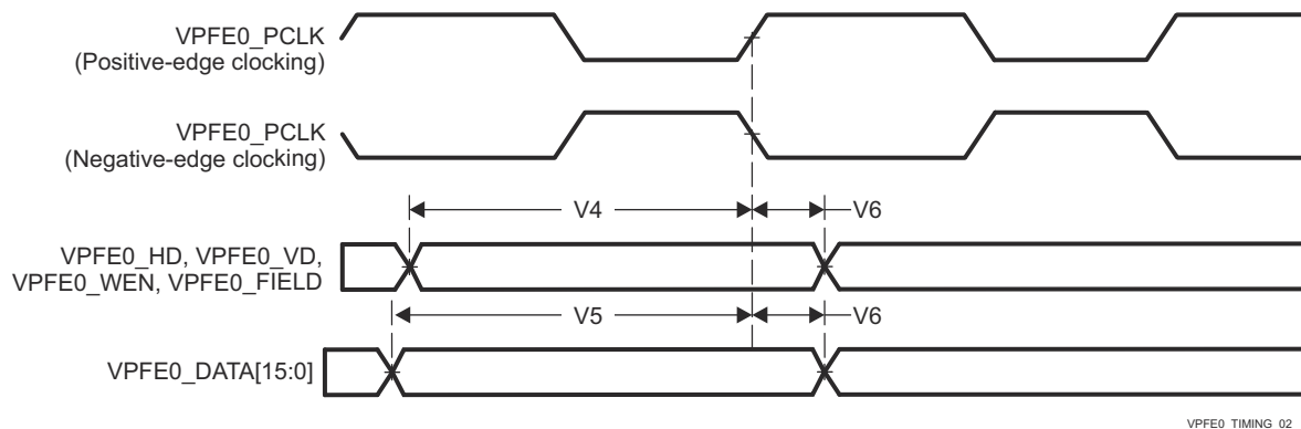
Figure 7-39. VPFE0 Timing Requirements
