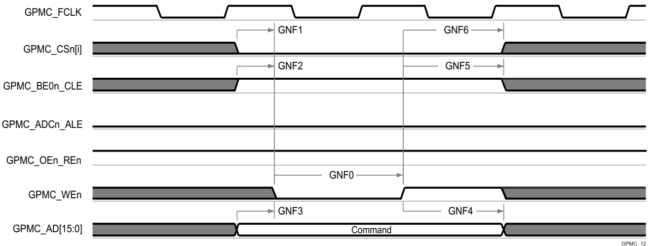
Figure 7-73. GPMC and NAND Flash — Command Latch Cycle
