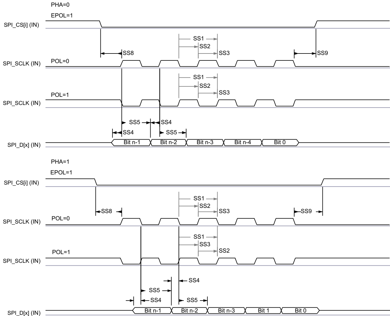
Figure 7-87. SPI Slave Mode Receive Timing
