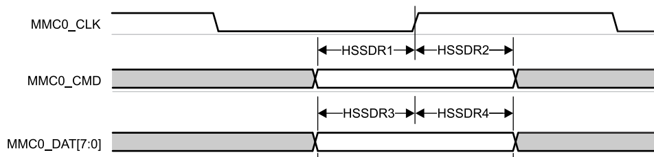
Figure 7-91. MMC0 – High Speed SDR Mode – Receive Mode
