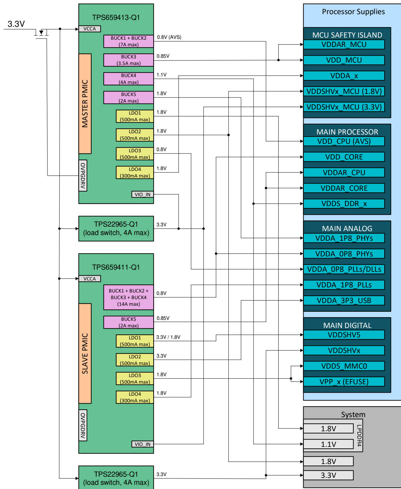
Figure 9-1. Power Connections with TPS659413-Q1 and TPS659411-Q1
