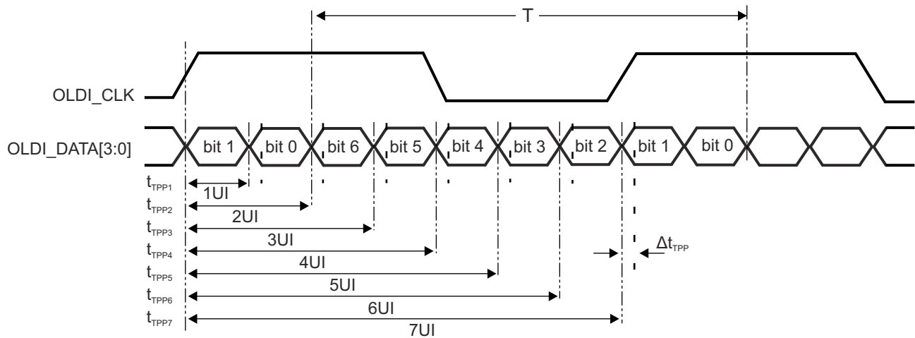
Figure 7-114. OLDI Transmitter Pulse Positions
