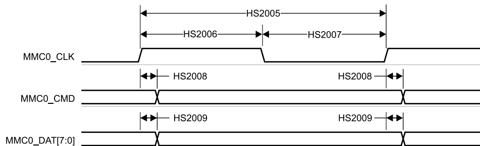
Figure 7-95. MMC0 – HS200 Mode – Transmit Mode
