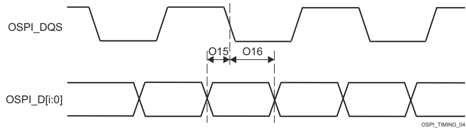
Figure 7-111. OSPI Timing Requirements – DDR, External Loopback Clock and DQS
