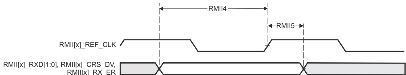
Figure 7-48. CPSW9G RMII[x]_RXD[1:0], RMII[x]_CRS_DV, RMII[x]_RXER Timing Requirements – RMII Mode
