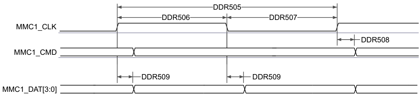
Figure 7-105. MMC1/2 – UHS-I DDR50 – Transmit Mode
