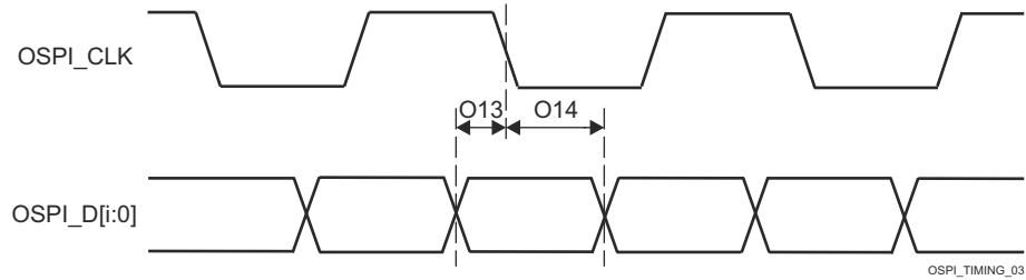
Figure 7-110. OSPI Timing Requirements – DDR, No Loopback Clock and Internal Pad Loopback Clock
