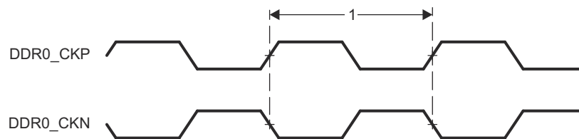
Figure 7-52. DDRSS Memory Interface Clock Timing
