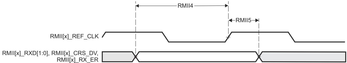
Figure 7-42. CPSW2G RMII[x]_RXD[1:0], RMII[x]_CRS_DV, RMII[x]_RX_ER Timing Requirements – RMII Mode
