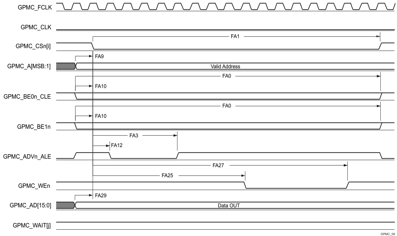
Figure 7-70. GPMC and NOR Flash — Asynchronous Write — Single Word
