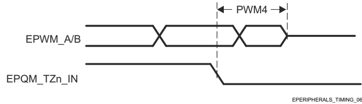
Figure 7-60. EPWM_A/B and ePWM_TZn_IN Hi-Z Input Timings
