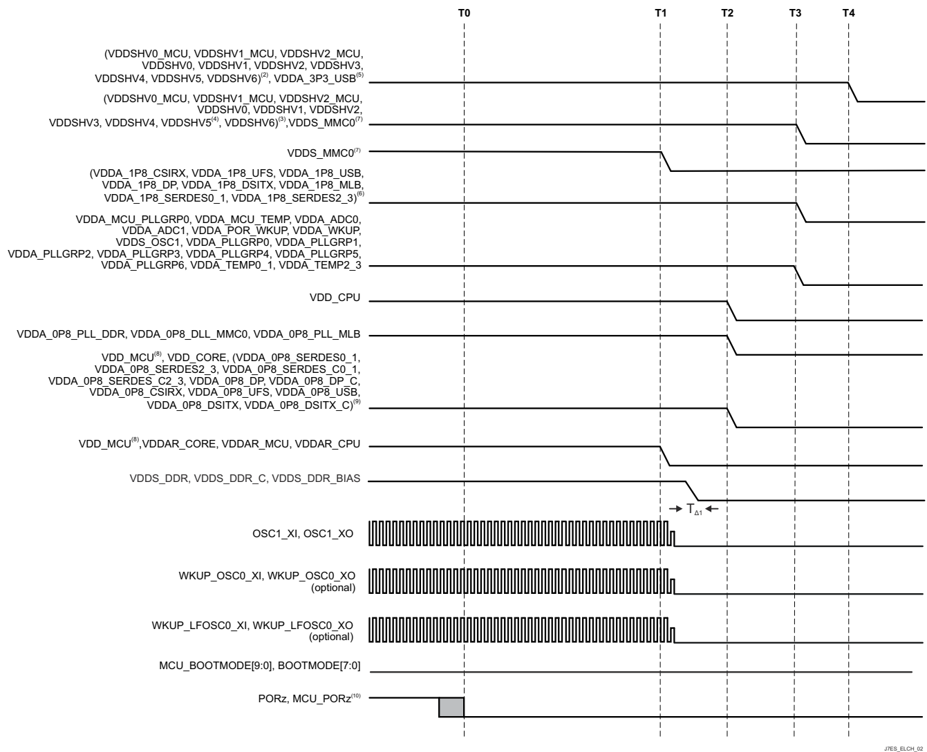
Figure 7-4. Combined MCU and Main Domains, Primary Power-Down Sequence
