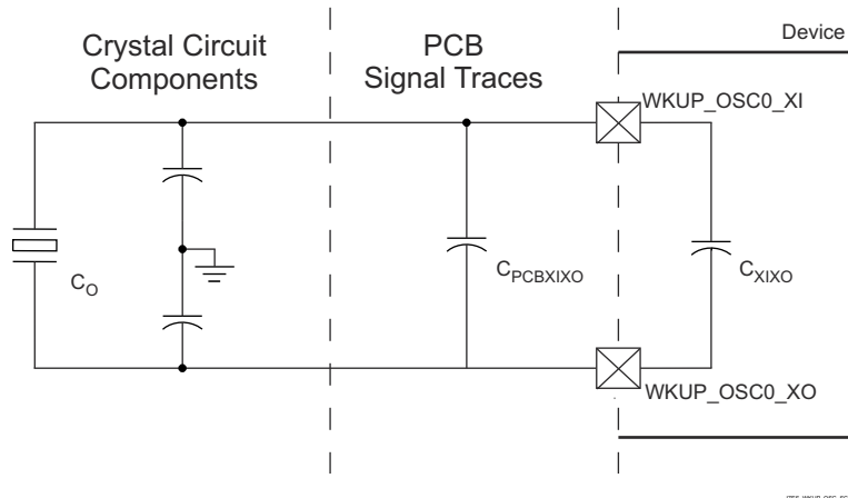
Figure 7-26. Shunt Capacitance
