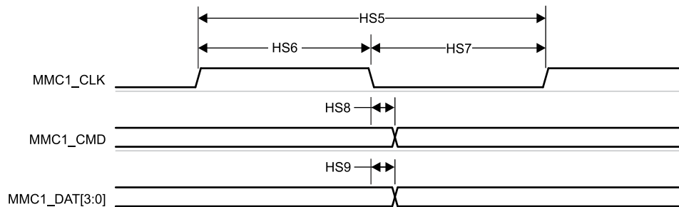
Figure 7-99. MMC1/2 – High Speed – Transmit Mode
