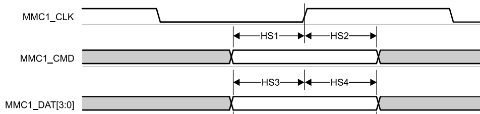
Figure 7-98. MMC1 /2– High Speed – Receive Mode
