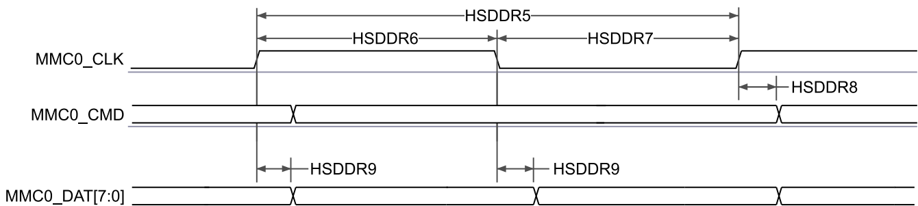
Figure 7-94. MMC0 – High Speed DDR Mode – Transmit Mode
