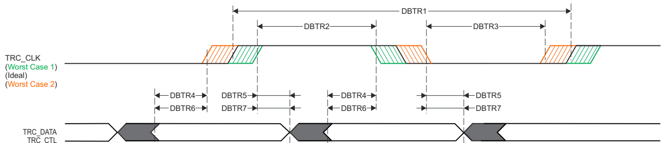
Figure 7-119. Trace Switching Characteristics
