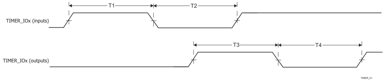
Figure 7-117. Timer Timing
