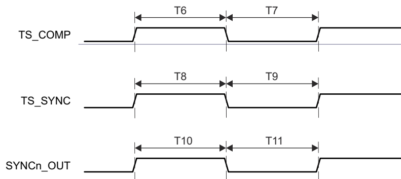
Figure 7-107. CPTS Switching Characteristics
