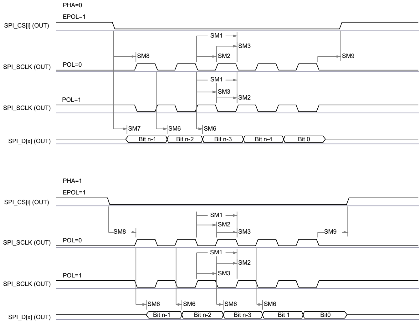
Figure 7-86. MCSPI Master Mode Transmit Timing
