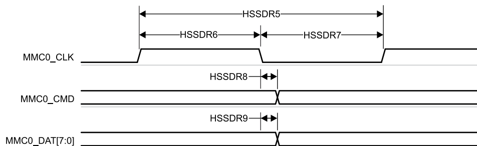
Figure 7-92. MMC0 – High Speed SDR Mode – Transmit Mode
