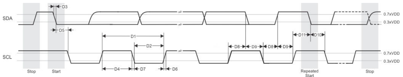
Figure 7-81. I3C Push-Pull Timing Requirements - HDR-DDR Mode
