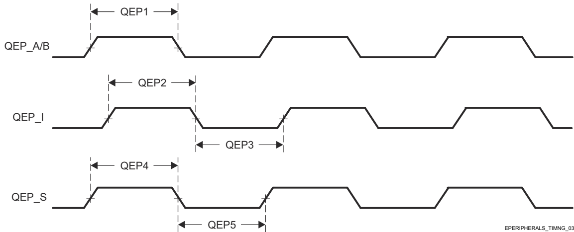
Figure 7-61. eQEP Input Timings
