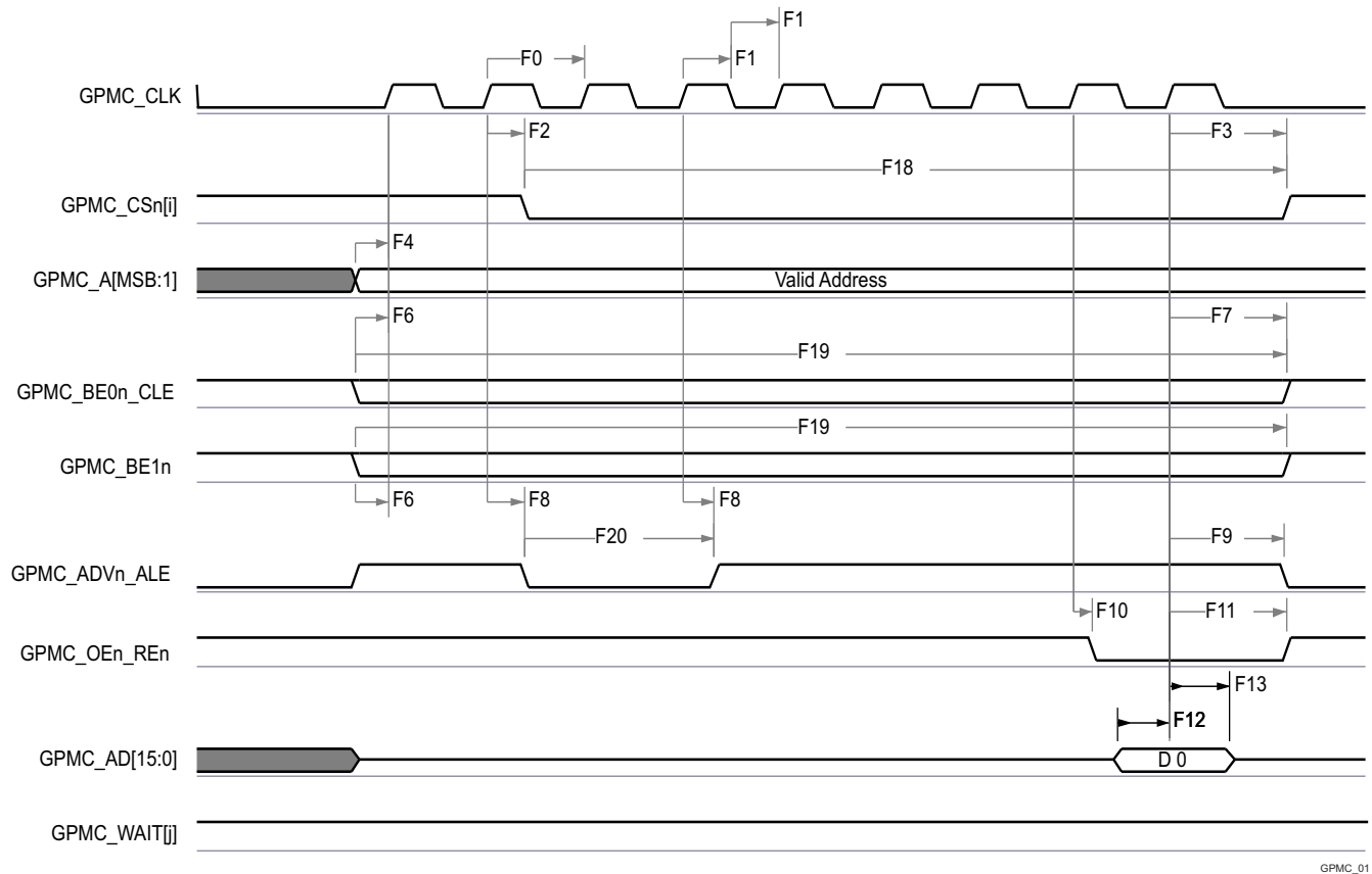
Figure 7-62. GPMC and NOR Flash — Synchronous Single Read (GPMCFCLKDIVIDER = 0)
