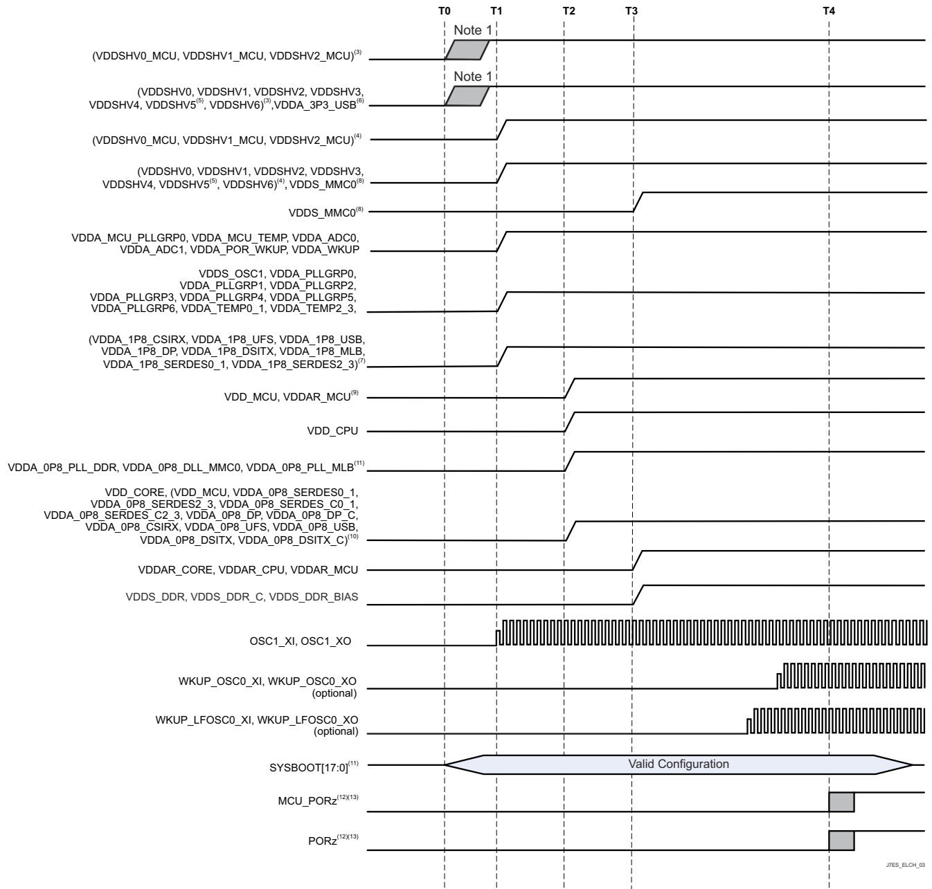
Figure 7-5. Independent MCU and Main Domains, Primary Power-Up Sequence
