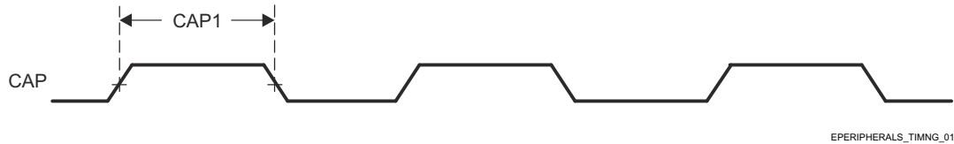
Figure 7-55. eCAP Input Timings
