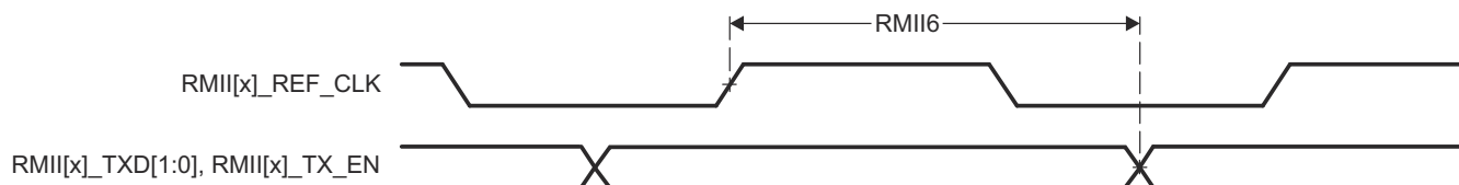
Figure 7-49. RMII[x]_TXD[1:0], and RMII[x]_TX_EN Switching Characteristics – RMII Mode
