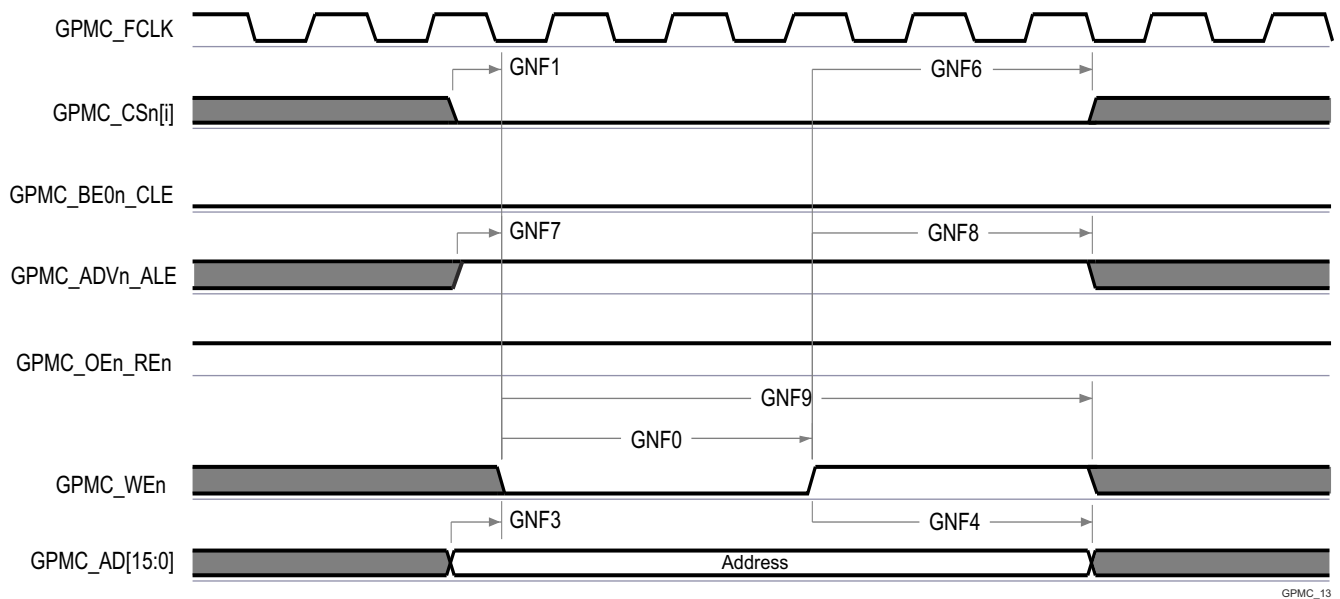
Figure 7-74. GPMC and NAND Flash — Address Latch Cycle
