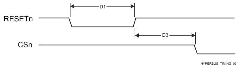
Figure 7-79. HyperBus Timing Diagrams – Reset
