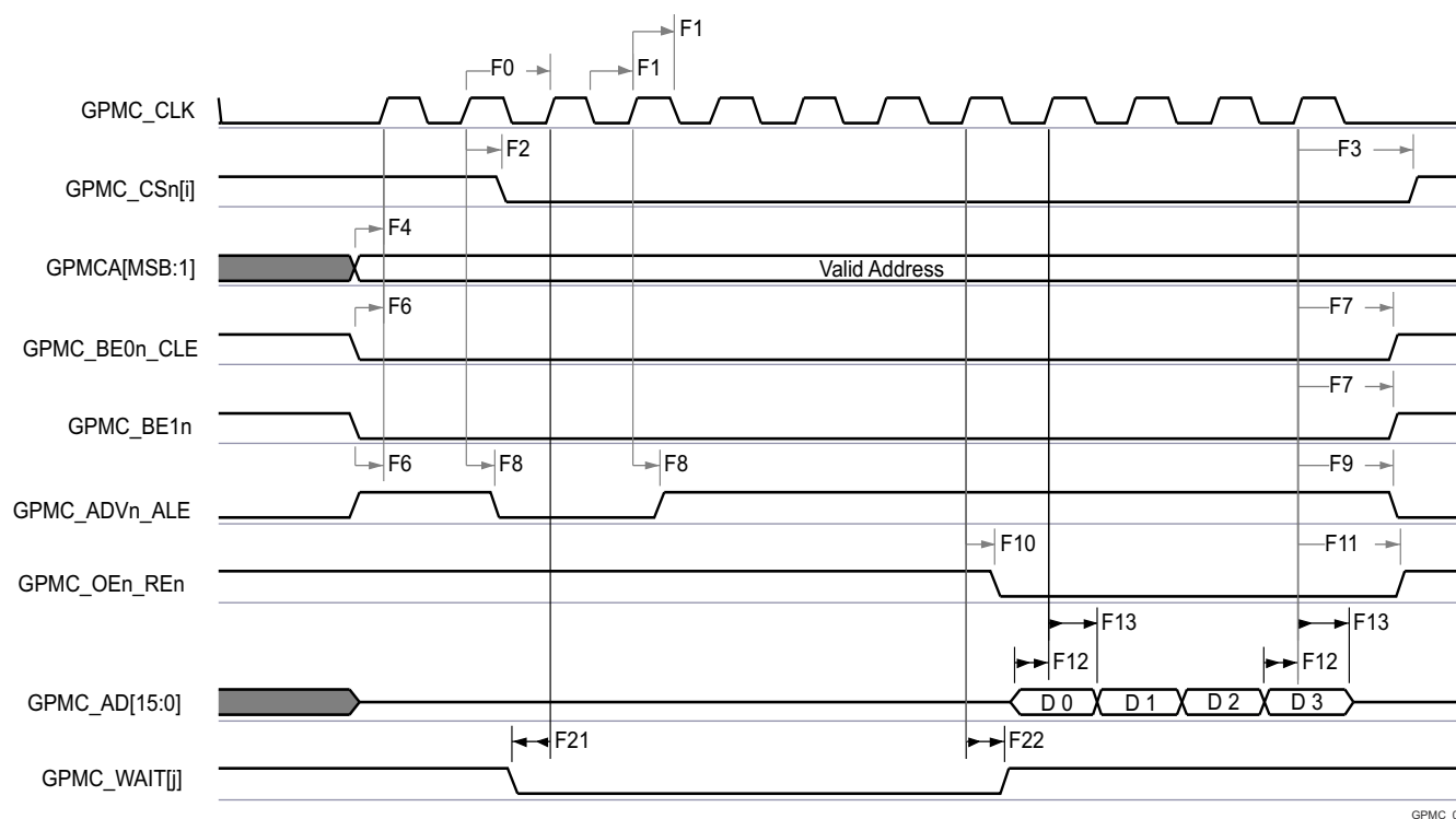
Figure 7-63. GPMC and NOR Flash — Synchronous Burst Read — 4x16-bit (GPMCCLKDIVIDER = 0)
