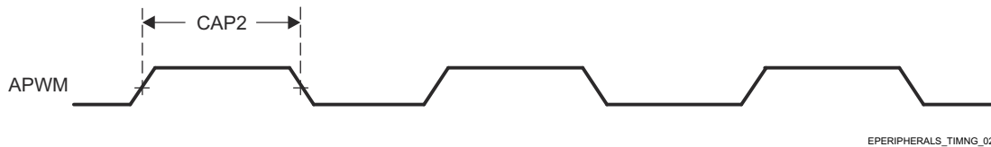
Figure 7-56. eCAP Output Timings
