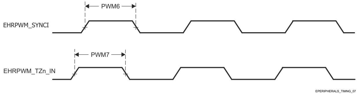
Figure 7-57. ePWM_SYNCI and ePWM_TZn_IN Output Timings
