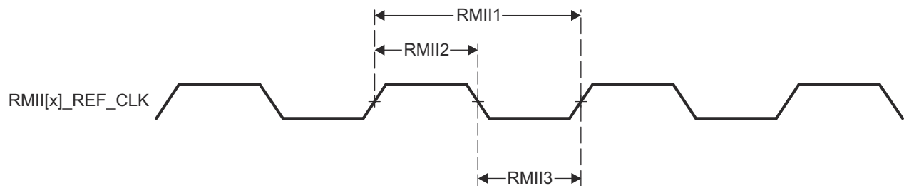
Figure 7-41. CPSW2G RMII[x]_REFCLK Timing Requirements – RMII Mode
