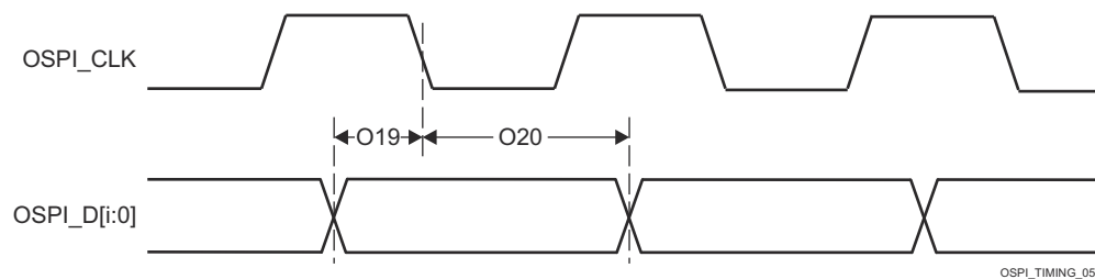
Figure 7-112. OSPI Timing Requirements – SDR, No Loopback Clock and Internal Pad Loopback Clock
