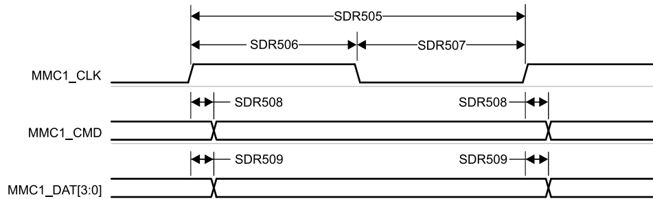
Figure 7-104. MMC1/2 – UHS-I SDR50 – Transmit Mode
