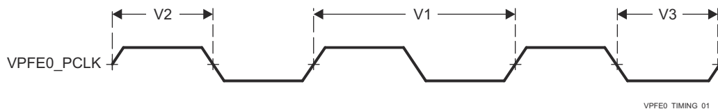
Figure 7-38. VPFE0 Clock Signal Requirement
