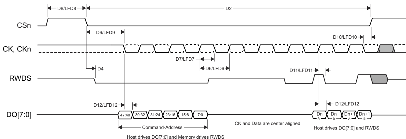
Figure 7-77. HyperBus Timing Diagrams – Transmitter Mode
