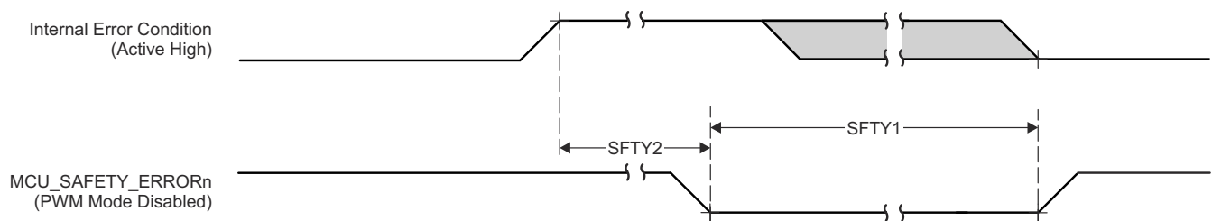
Figure 7-18. MCU_SAFETY_ERRORn Switching Characteristics
