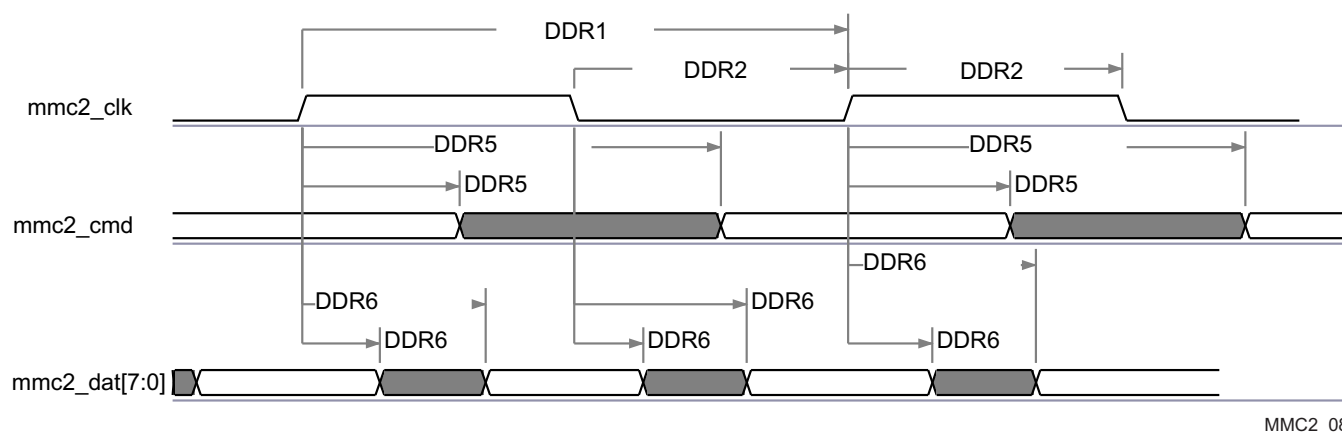
Figure 5-103. MMC/SD/SDIO in - High-Speed DDR JC64 - Transmitter Mode
