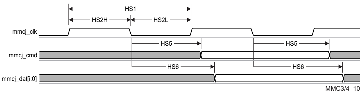
Figure 5-107. MMC/SD/SDIOj in - High Speed - Transmitter Mode
