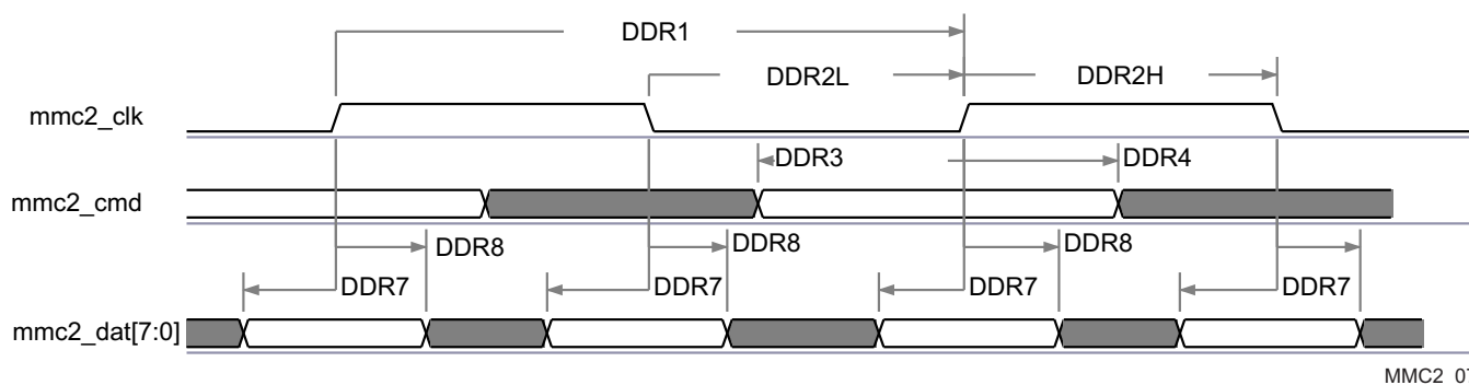
Figure 5-102. MMC/SD/SDIO in - High-Speed DDR JC64 - Receiver Mode
