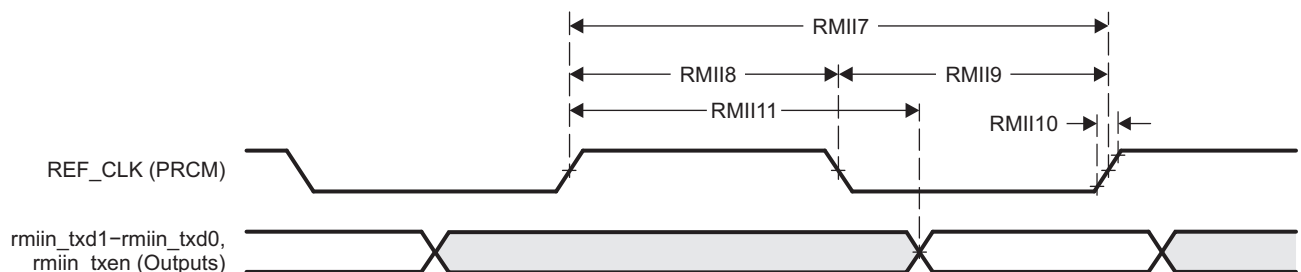
Figure 5-79. GMAC Transmit Interface Timing RMIIIn Operation
