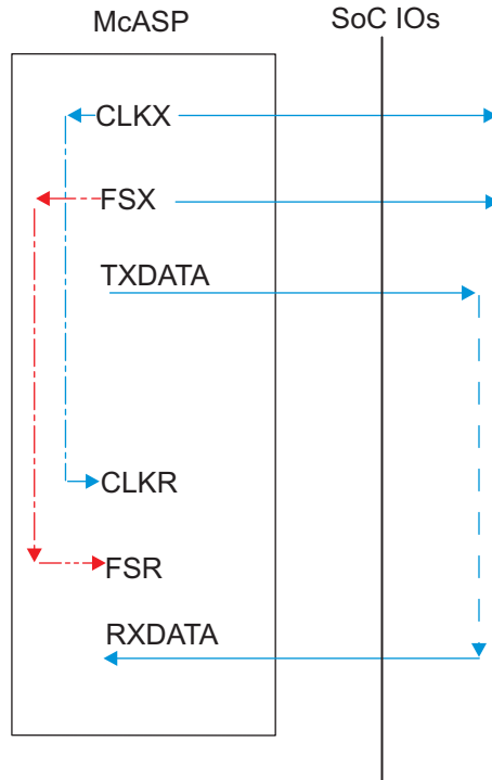
图 5-60. McASP1-8 CO-FO- – SYNC Mode
