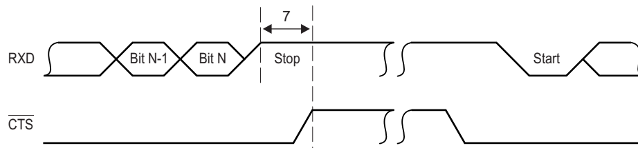
图 11-45. UART RTS (Request-to-Send Output) – Autoflow Timing Waveform
