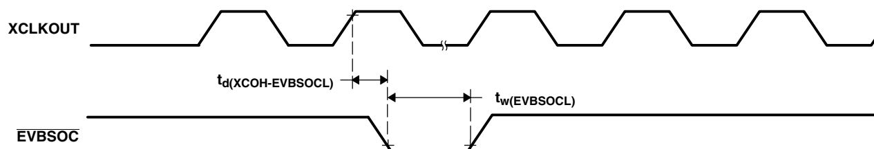
Figure 6–18. EVBSOC Timing
