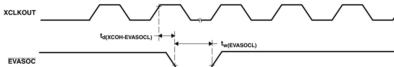
Figure 6–17. EVASOC Timing
