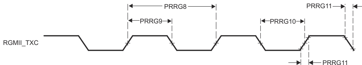
Figure 7-116. PRU_ICSSG RGMII_TXC Switching Characteristics
