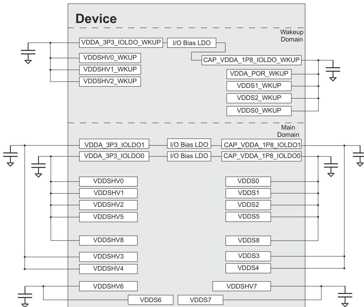
Figure 9-7. All VDDSHV[8:0], and VDDSHV[2:0]_WKUP Supplies Configured for 3.3 V Operation
