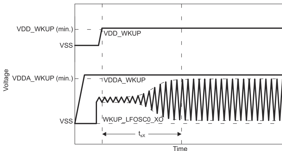
Figure 7-26. WKUP_LFOSC0 Start-up Time
