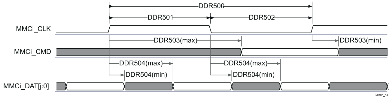
Figure 7-81. eMMC/SD/SDIO - High-Speed DDR - DDR50 - Transmit Mode
