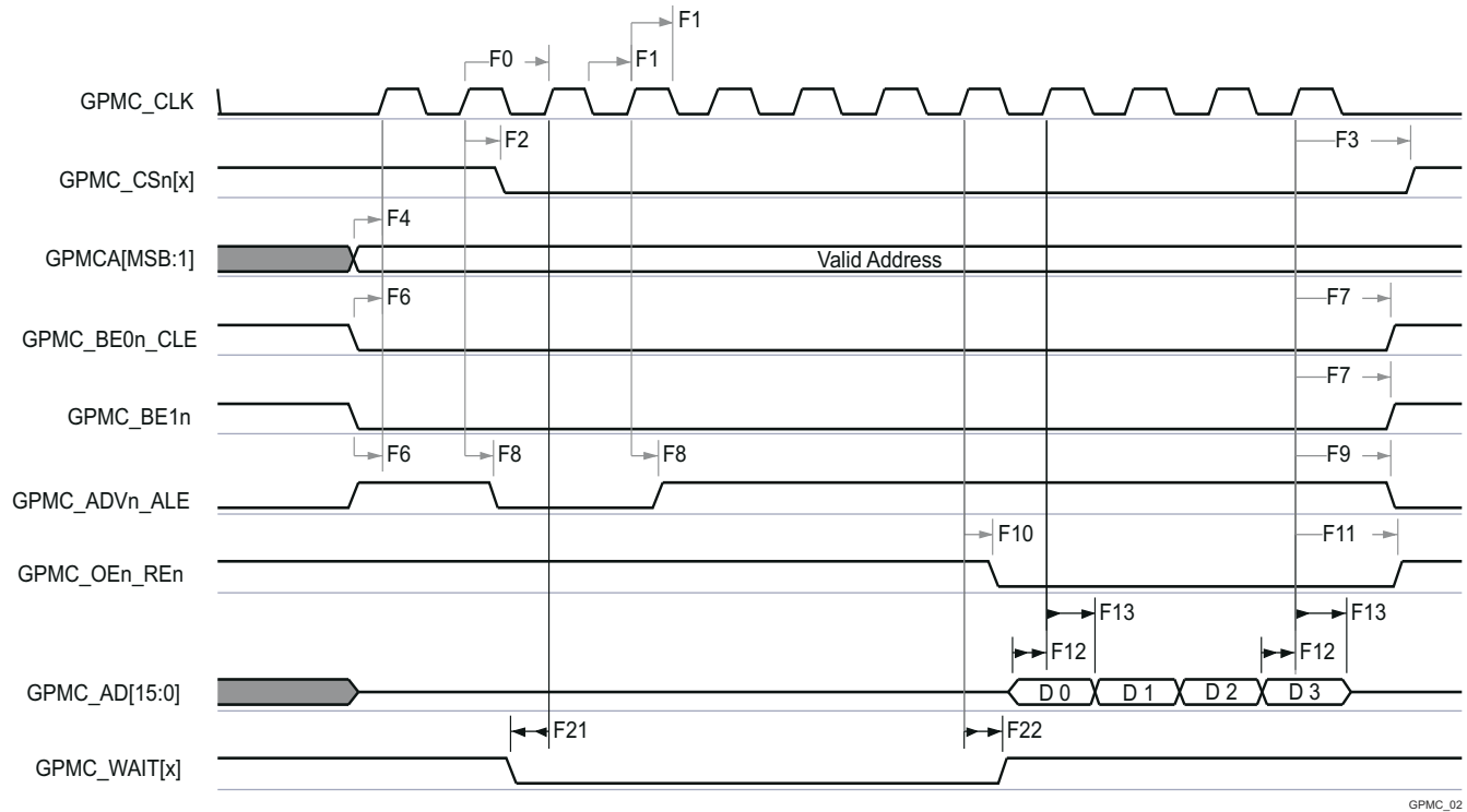
Figure 7-49. GPMC and NOR Flash—Synchronous Burst Read—4x16-bit (GpmcCLKDivider = 0)
