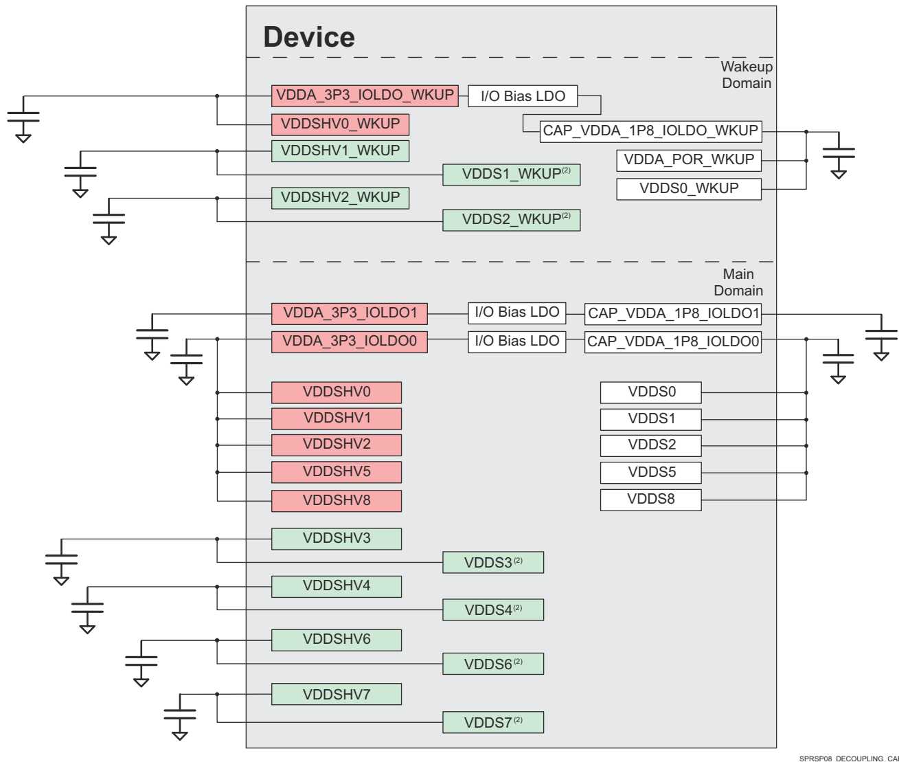
Figure 9-9. VDDSHV[8:0] and VDDSHV[2:0]_WKUP Supplies Configured for Combination of 1.8 V or 3.3 V Operation
