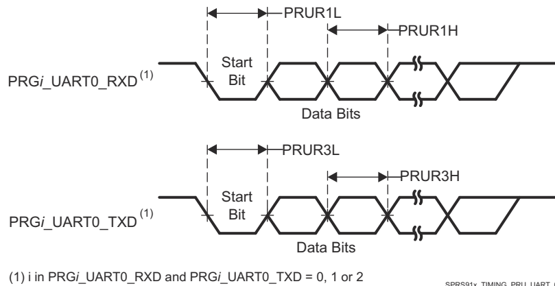
Figure 7-108. PRU_ICSSG UART Timing
