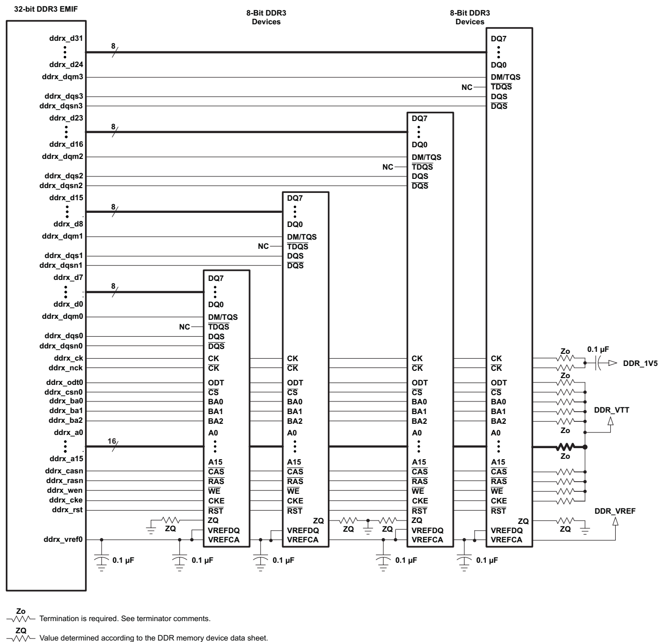
图 8-59. 32-Bit, One-Bank DDR3 Interface Schematic Using Four 8-Bit DDR3 Devices
