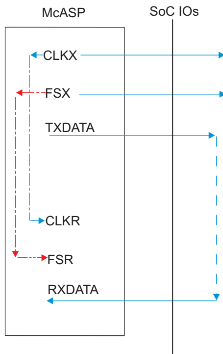
图 7-40. McASP1-8 CO-FO- – SYNC Mode
