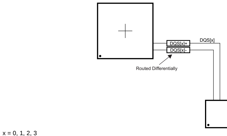
Figure 5-85. DQS[x] Routing
