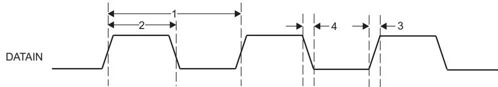
Figure 5-123. PRU-ICSS PRU Shift In Timing
