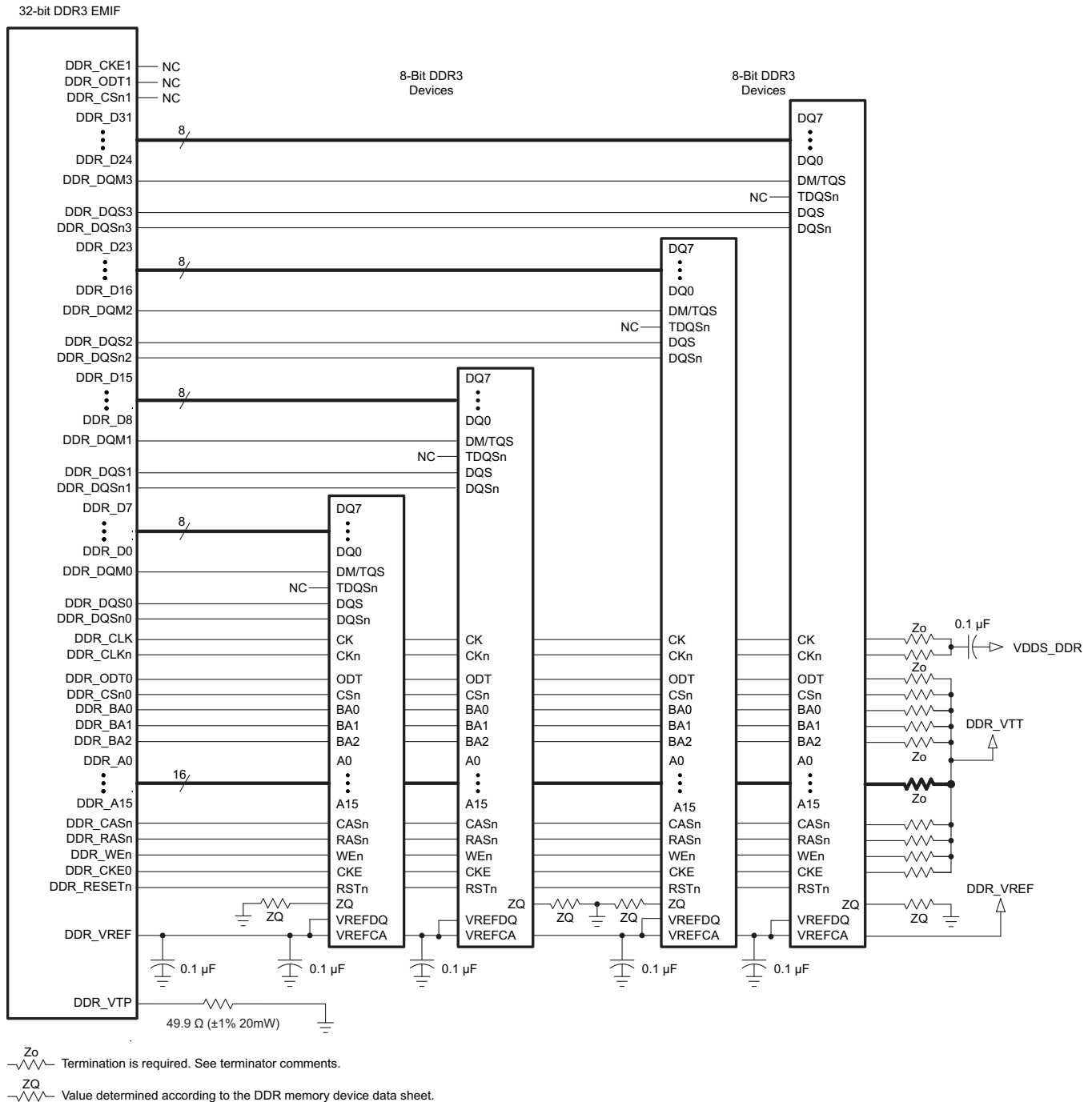
Figure 5-53. 32-Bit DDR3 Interface Using Four 8-Bit DDR3 Devices With V_{\Pi} Termination
