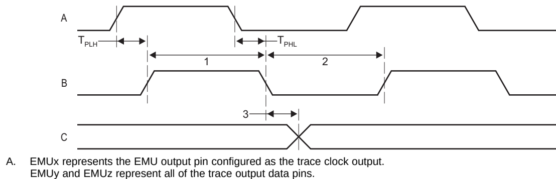
Figure 5-31. Trace Timing
