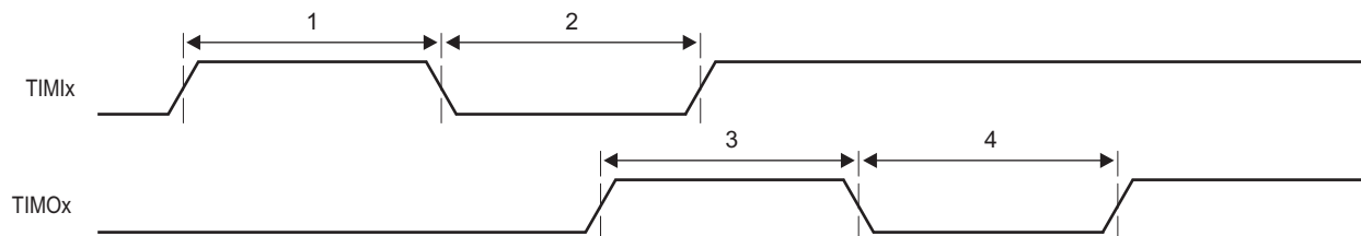
Figure 5-23. Timer Timing
