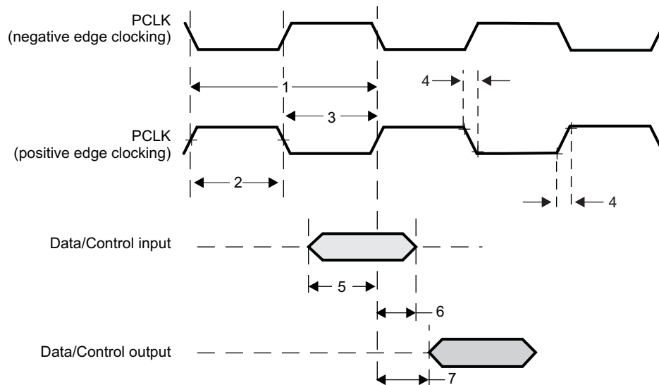
Figure 8-35. ISSCAM Timings
