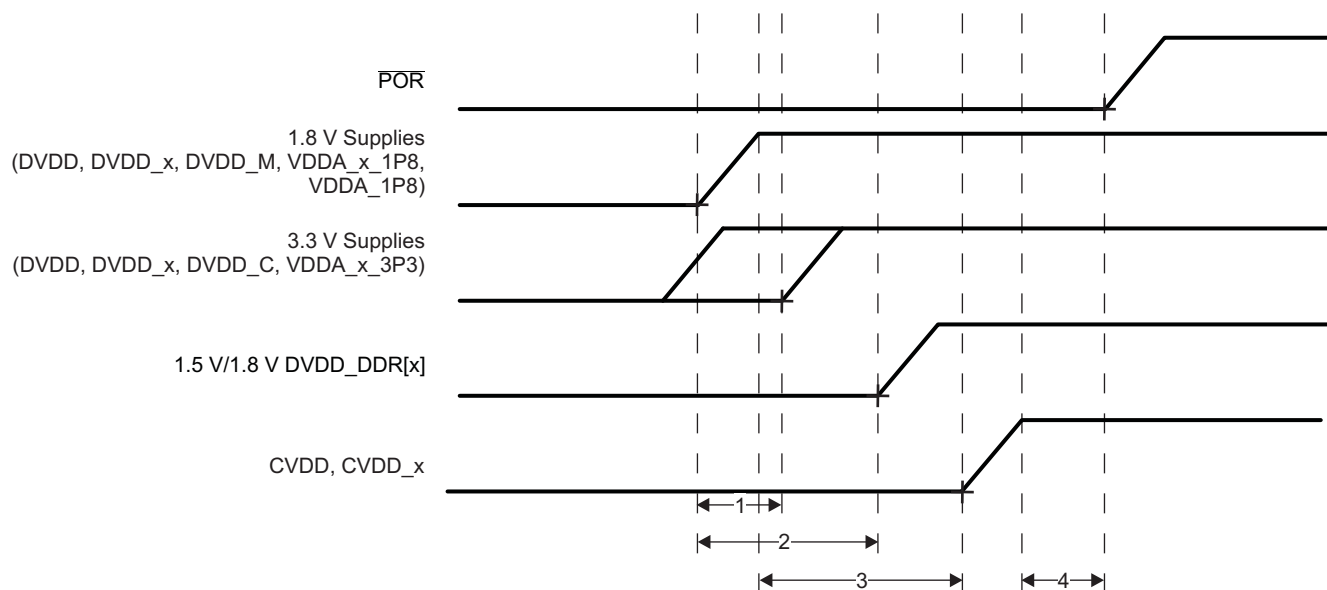
Figure 7-1. Power-Up Sequence
