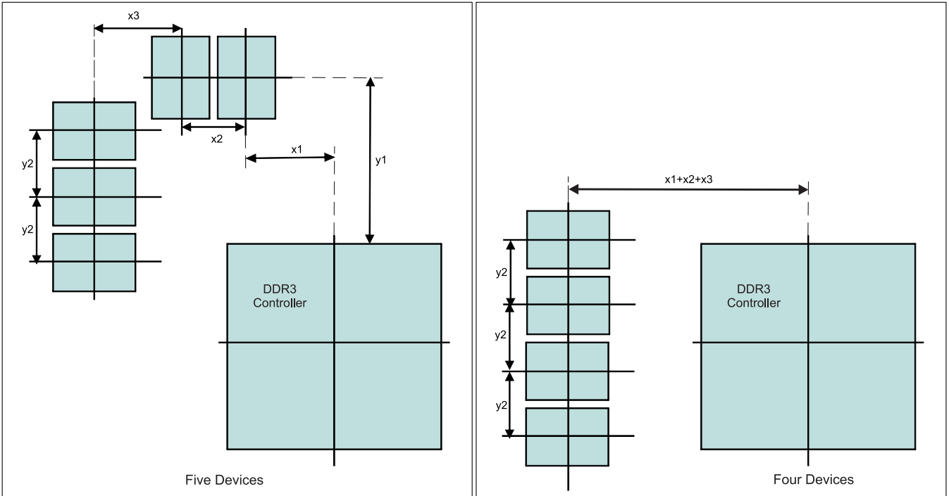
图 8-43. Placement Specifications
