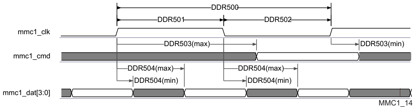
图 7-75. SDRAM - High Speed SD - DDR - Data/Command Transmit
