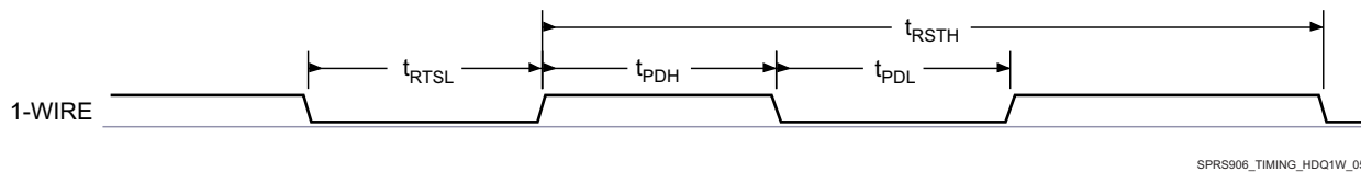
图 7-29. 1-Wire-Break (Reset)
