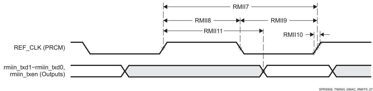
图 7-58. GMAC Transmit Interface Timing RMIIIn Operation
