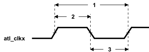
图 7-93. ATL_CLKOUTx Timing
