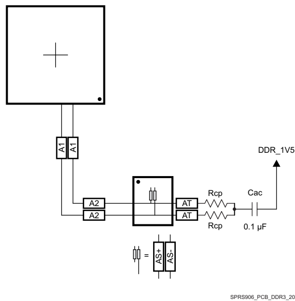
图 8-59. CK Routing for One DDR3 Device
