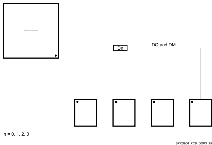
图 8-64. DQ/DM Routing With Any Number of Allowed DDR3 Devices
