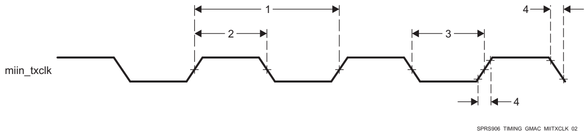
图 7-53. Clock Timing (GMAC Transmit) - MII operation
