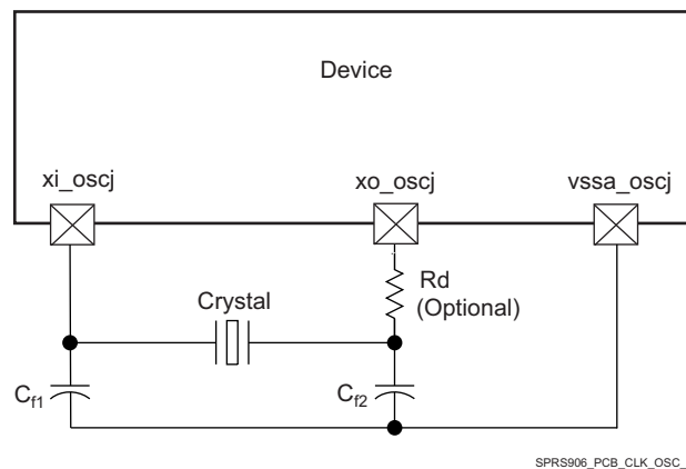
图 8-39. Grounding Scheme for High-Frequency Clock
