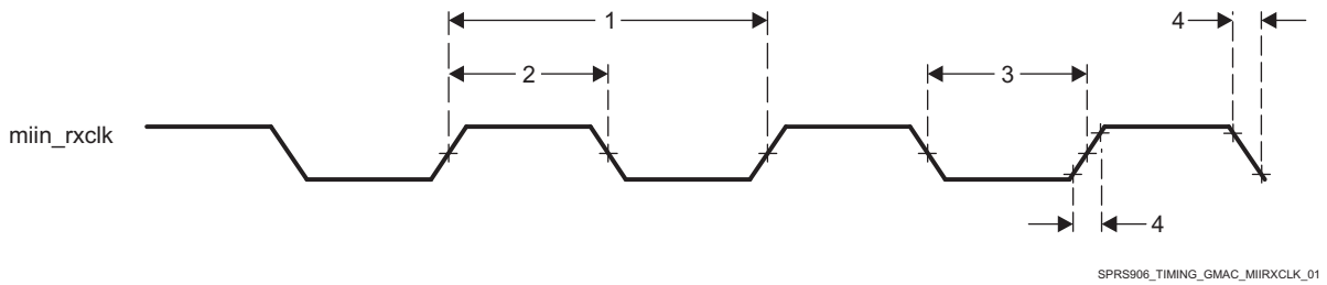
图 7-52. Clock Timing (GMAC Receive) - MII operation
