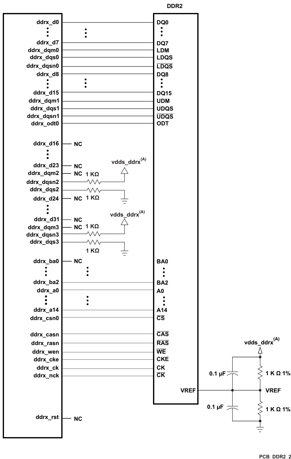
图 7-25. 16-Bit DDR2 High-Level Schematic
