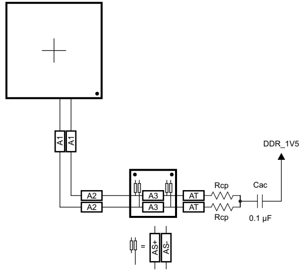
图 7-45. CK Routing for Two Mirrored DDR3 Devices
