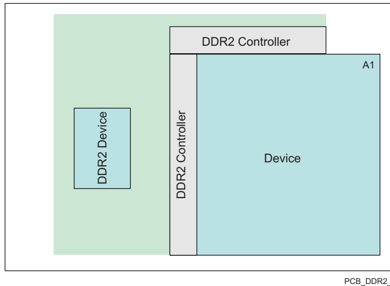
图 7-27. DDR2 Keepout Region
