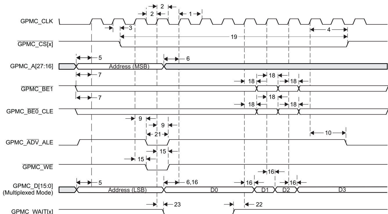
Figure 8-27. GPMC Non-Multiplexed NOR Flash - Synchronous Burst Write (GPMCCLKDIVIDER = 0)
