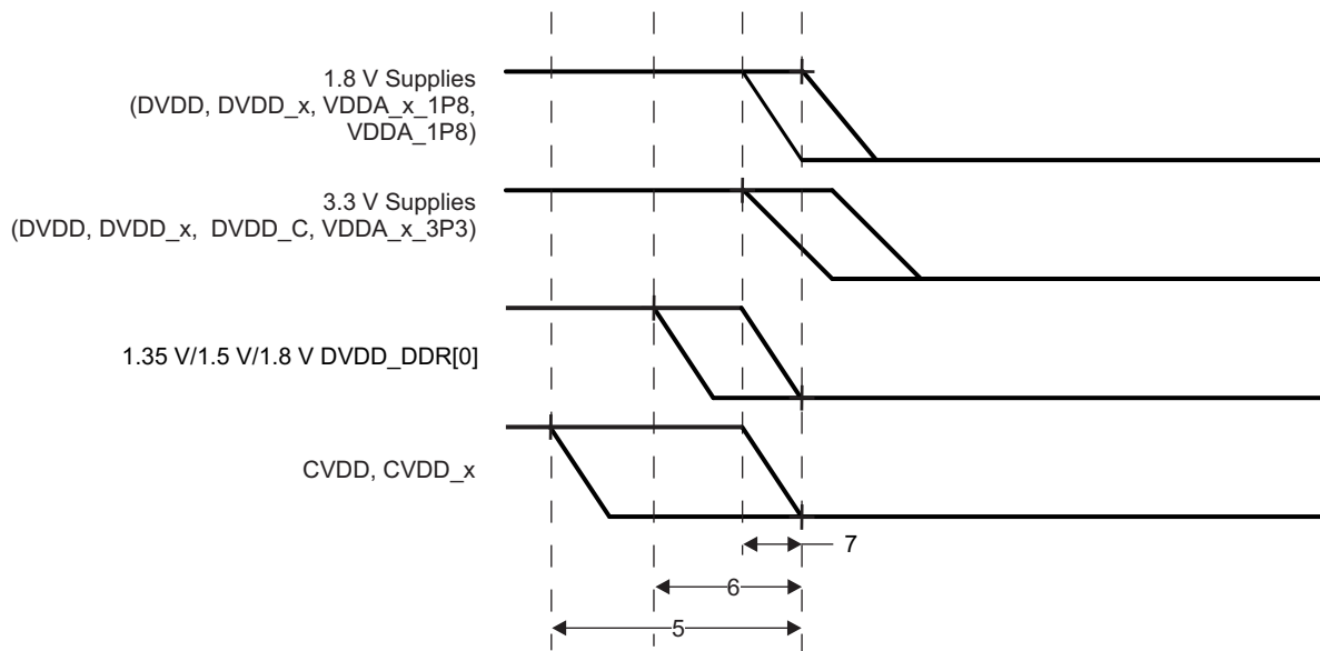
Figure 7-2. Power-Down Sequence
