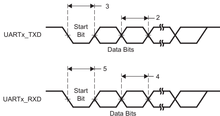
Figure 8-98. UART Timing
