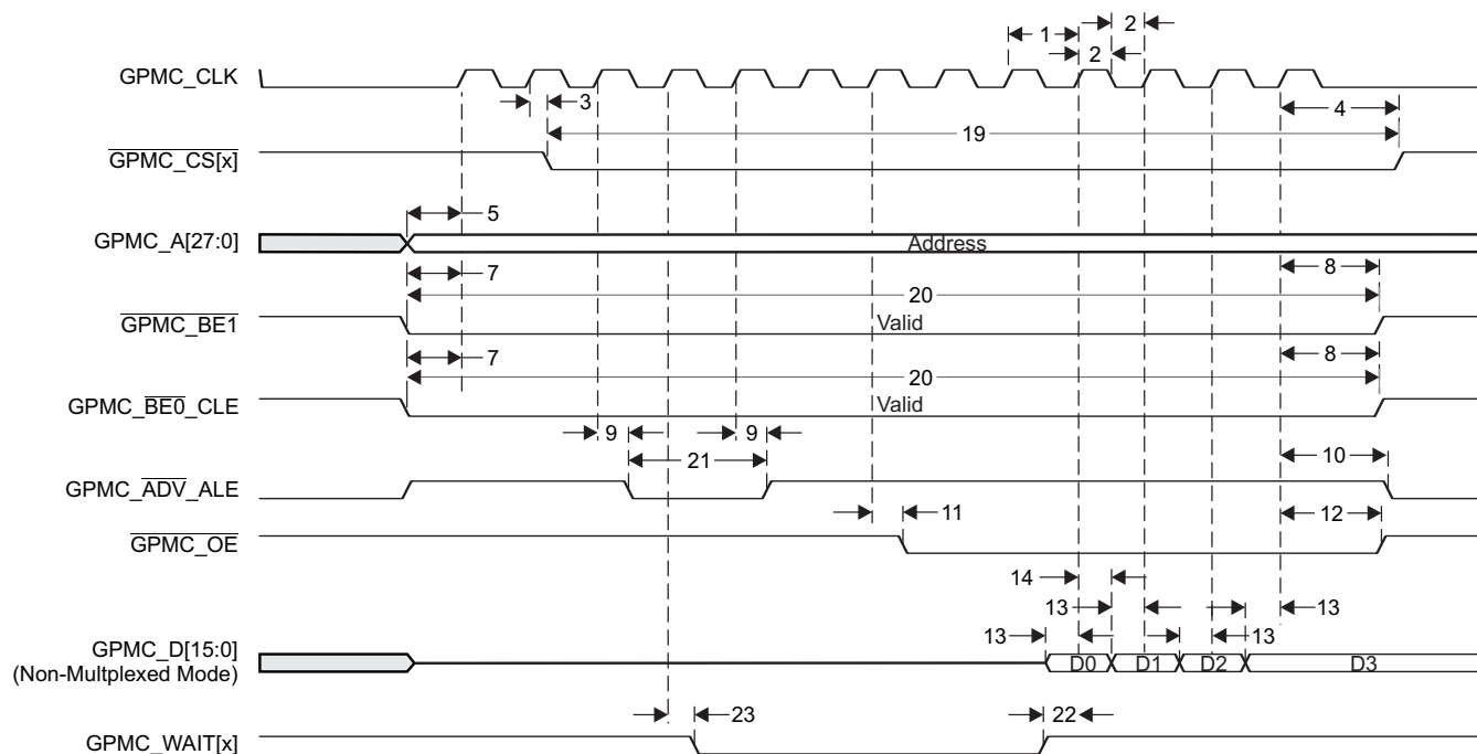
Figure 8-23. GPMC Non-Multiplexed NOR Flash - 14x16-bit Synchronous Burst Read (GPMCFCLKDIVIDER = 0)
