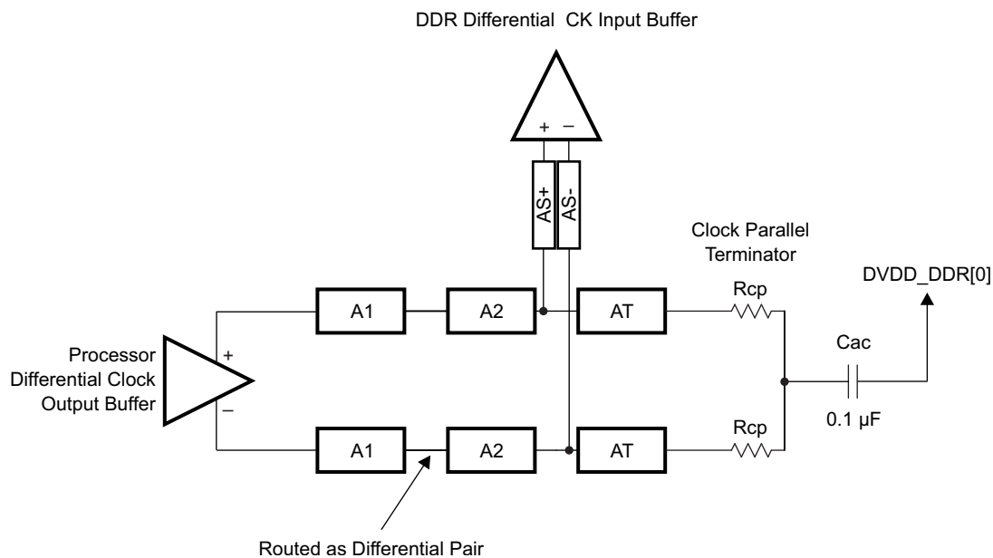
Figure 8-73. CK Topology for One DDR3 Device
