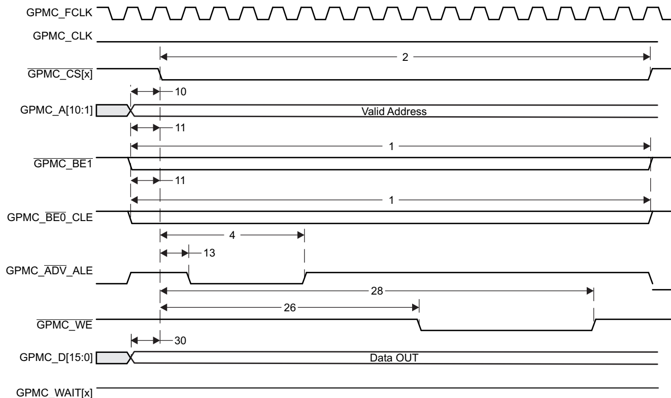
Figure 8-31. GPMC/Non-Multiplexed NOR Flash - Asynchronous Write - Single Word Timing
