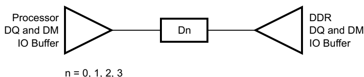
Figure 8-78. DQ/DM Topology
