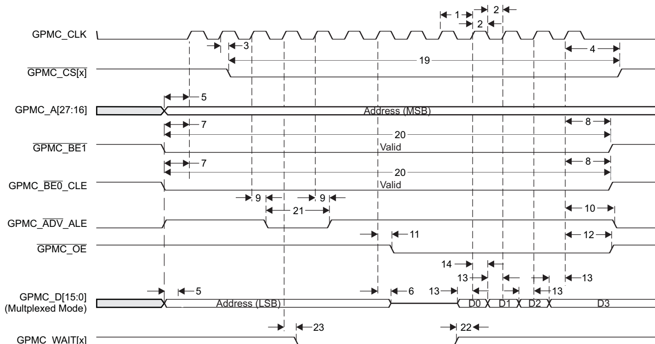
Figure 8-26. GPMC Multiplexed NOR Flash - 14x16-bit Synchronous Burst Read (GPMCCLKDIVIDER = 0)
