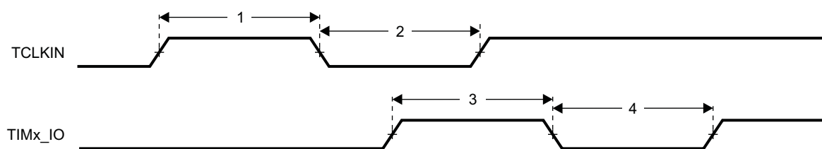
Figure 8-97. Timer Timing
