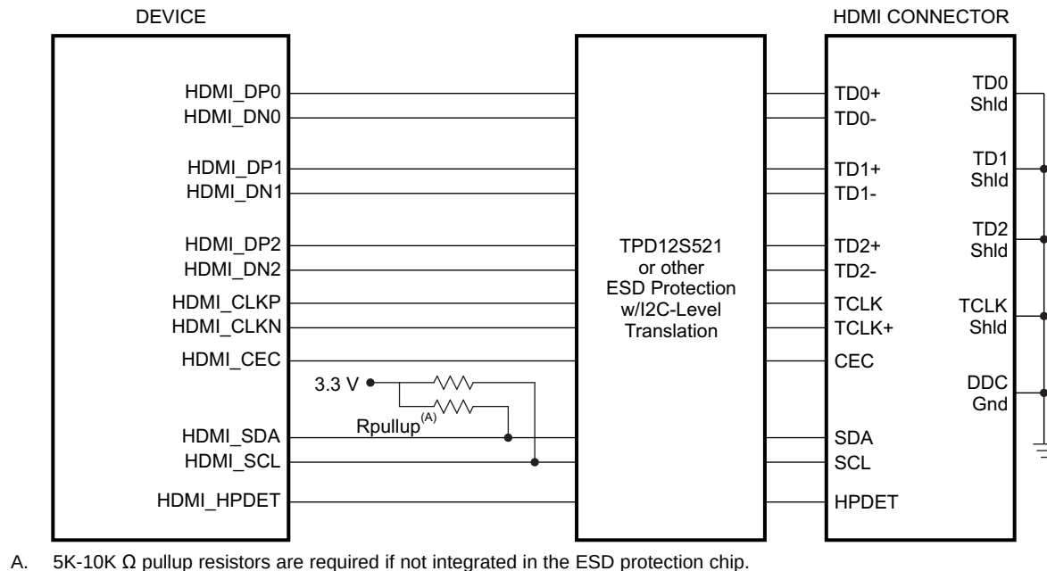
Figure 8-38. HDMI Interface High-Level Schematic
