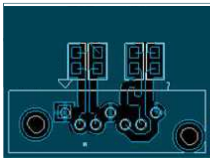
Figure 8-91. SATA Routing
