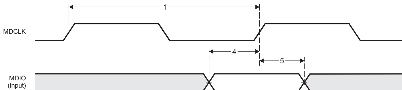
Figure 8-19. MDIO Input Timing
