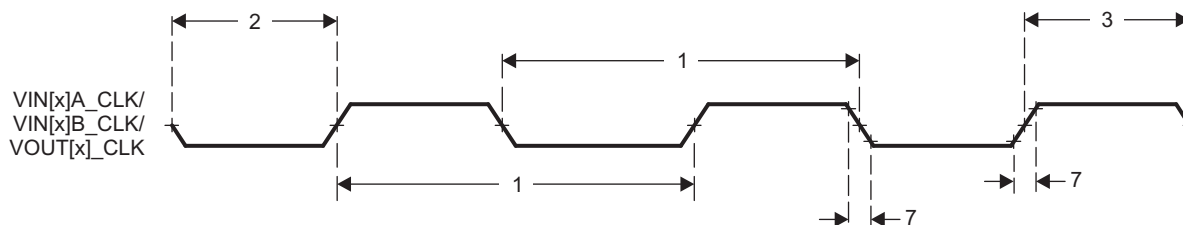
Figure 8-39. HDVPSS Clock Timing
