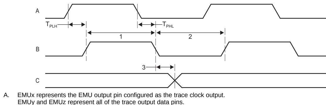
Figure 8-55. Trace Timing
