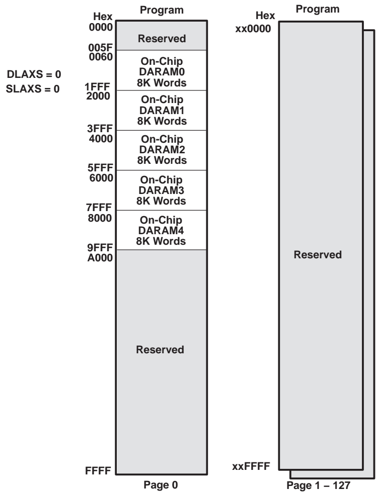
Figure 3–17. On-Chip DMA Memory Map for Program Space (DLAXS = 0 and SLAXS = 0)
