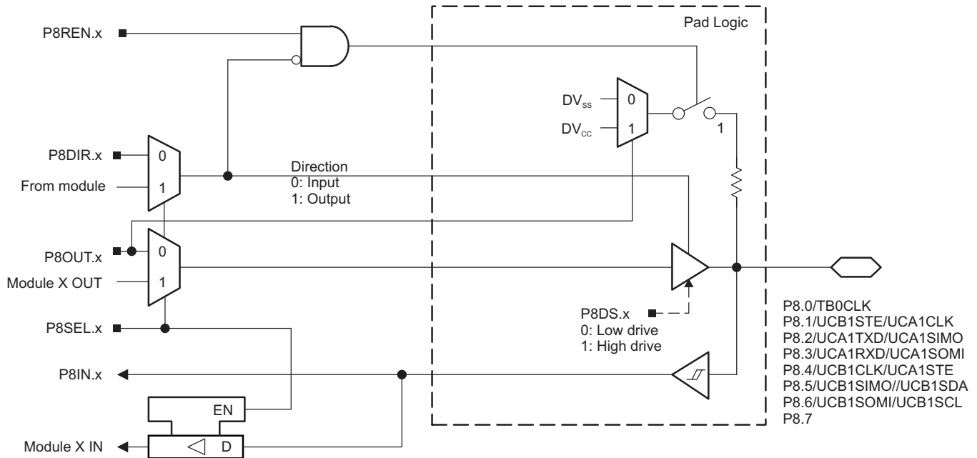
图 6-12. Port P8 (P8.0 to P8.7) Diagram
