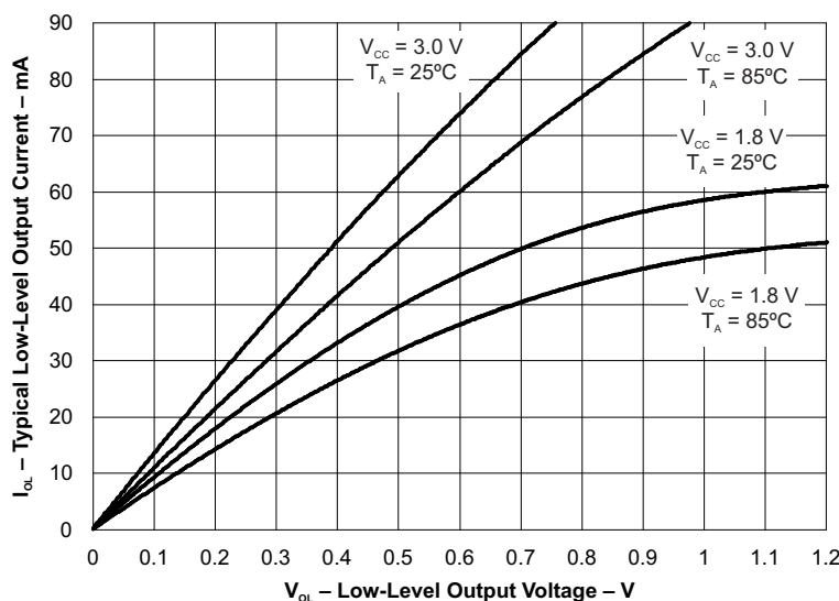
图 5-23. Ports PU.0, PU.1 Typical Low-Level Output Characteristics
