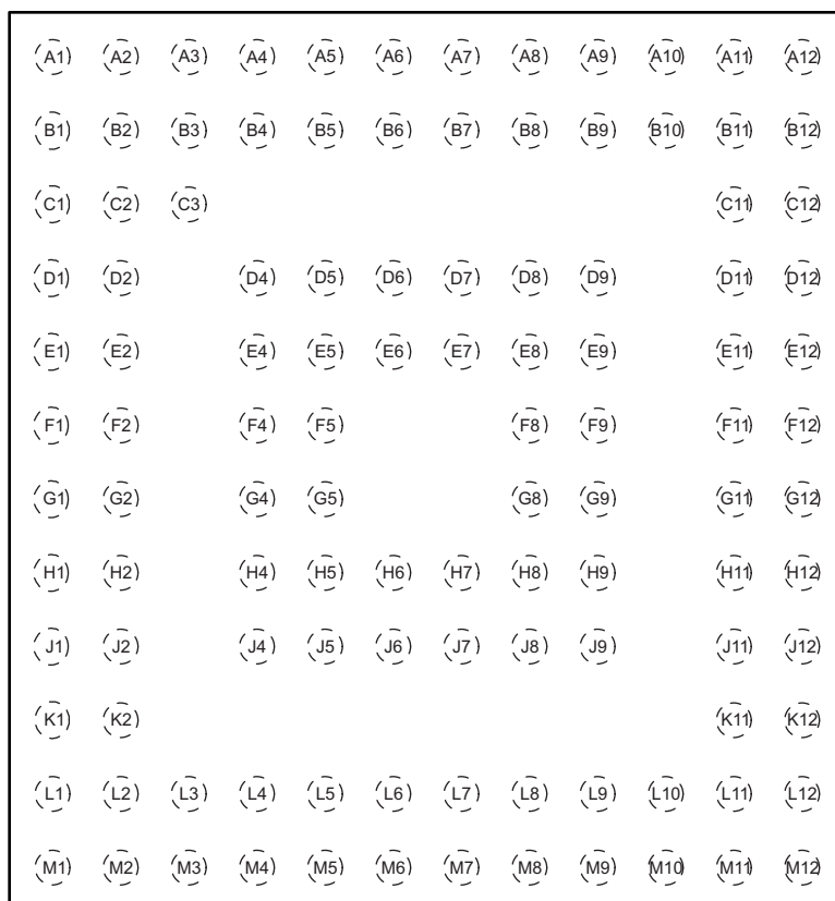
Figure 4-3. 113-Pin ZQW Package (Top View) – MSP430F5338, MSP430F5336, MSP430F5335, MSP430F5333
