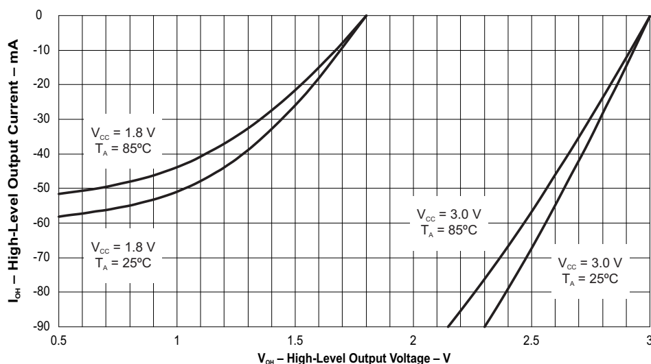
图 5-24. Ports PU.0, PU.1 Typical High-Level Output Characteristics
