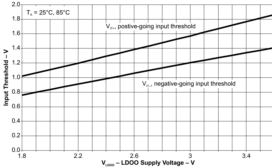
图 5-25. Ports PU.0, PU.1 Typical Input Threshold Characteristics
