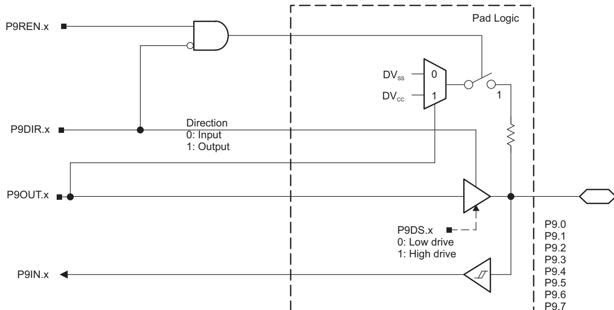
图 6-13. Port P9 (P9.0 to P9.7) Diagram
