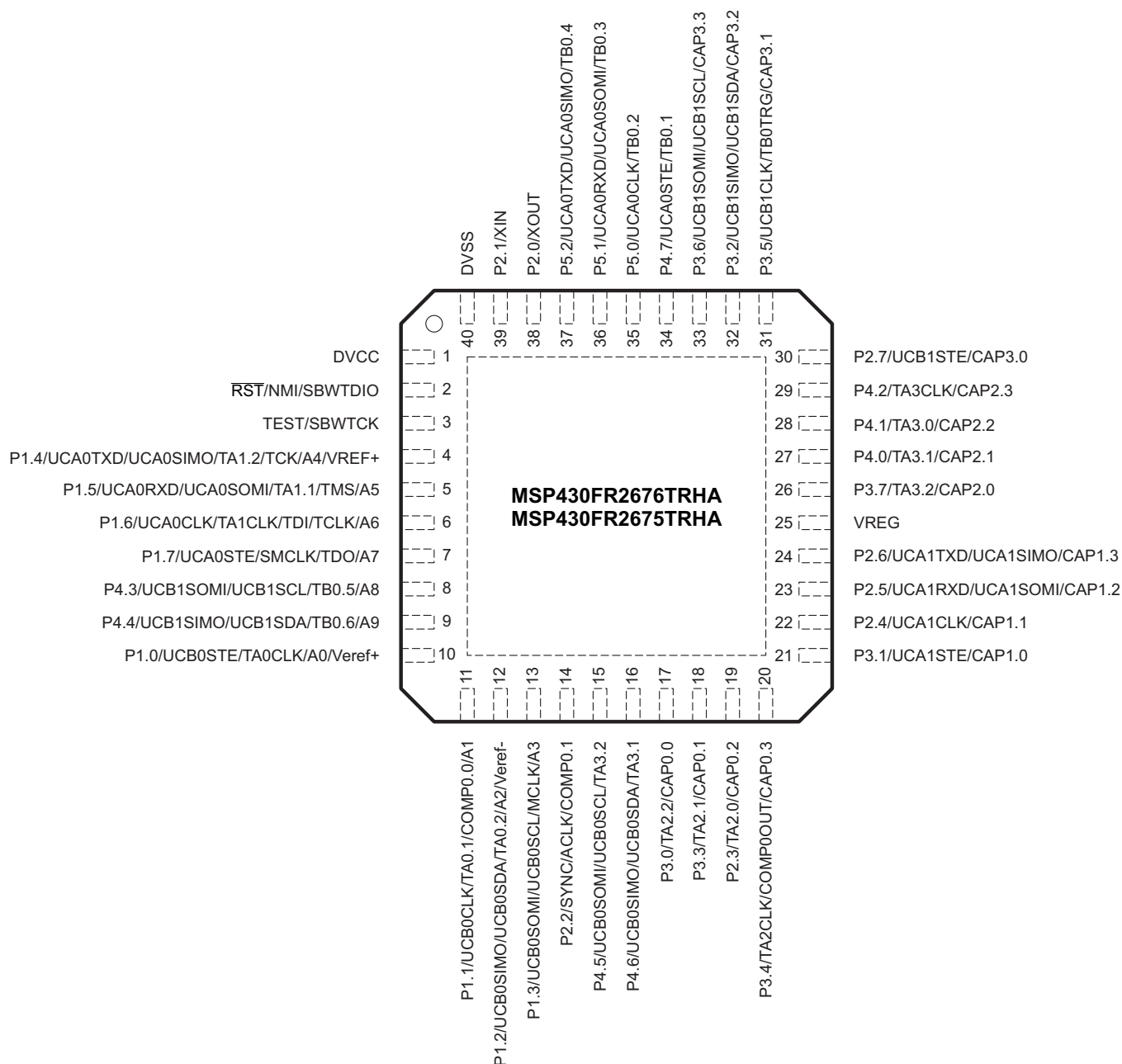
Figure 4-2. 40-Pin RHA Package (Top View)
