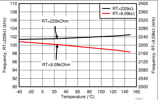
图 2. Frequency vs Temperature
