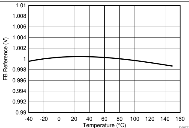
图 7. FB Reference vs Temperature
