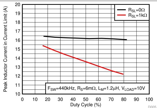
图 5. Peak Current Limit vs Duty Cycle
