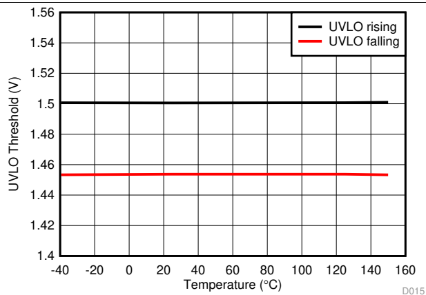
图 15. UVLO Threshold vs Temperature
