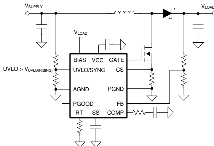
图 22. Decrease the Minimum Operating Voltage After Start-Up
