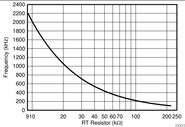
图 1. Frequency vs RT Resistance
