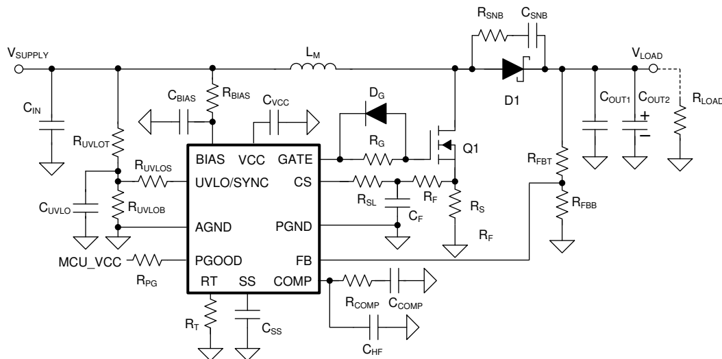
37. Typical Boost Converter Circuit With Optional Components
