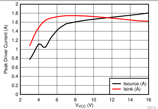
图 14. Peak Driver Current vs V_{CC}
