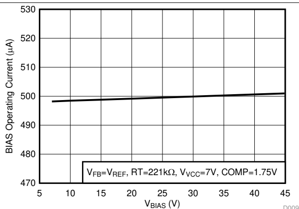
图 9. I_{\text{OPERATING}}(\text{BIAS}) including RT current vs V_{\text{BIAS}}
