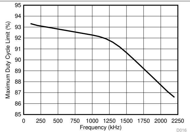
图 16. Maximum Duty Cycle vs Frequency
