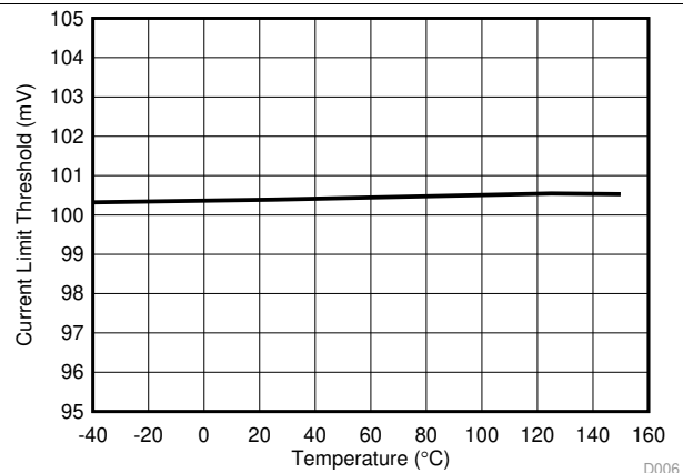
图 6. Current Limit Threshold vs Temperature
