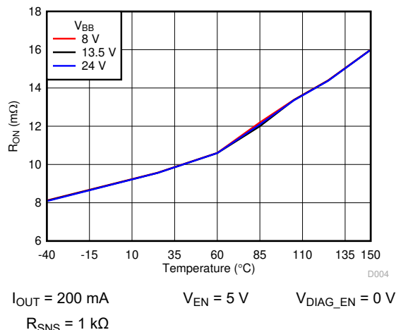
Figure 7-5. On Resistance ( R_{ON} ) vs Temperature
