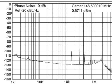
Figure 2. CLKout1 Phase Noise
