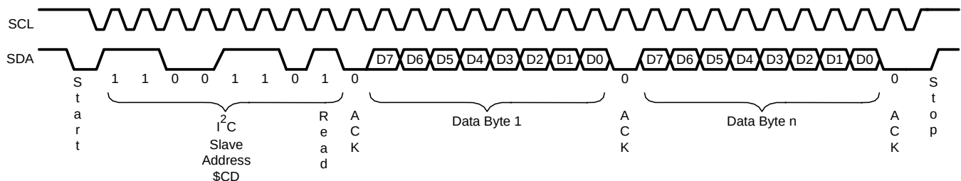
Figure 21. Read Sequence — Data Read Transfer
