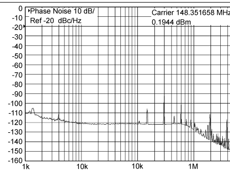
Figure 4. CLKout2 Phase Noise
