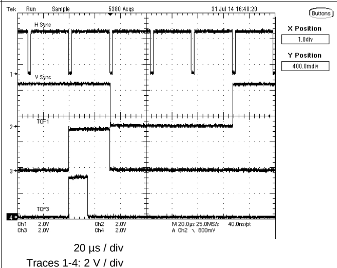
Figure 25. TOF1 Falling Edge Alignment with HSync and VSync Reference Timing
