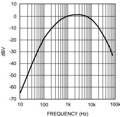
Figure 22. A-Weighted Filter
