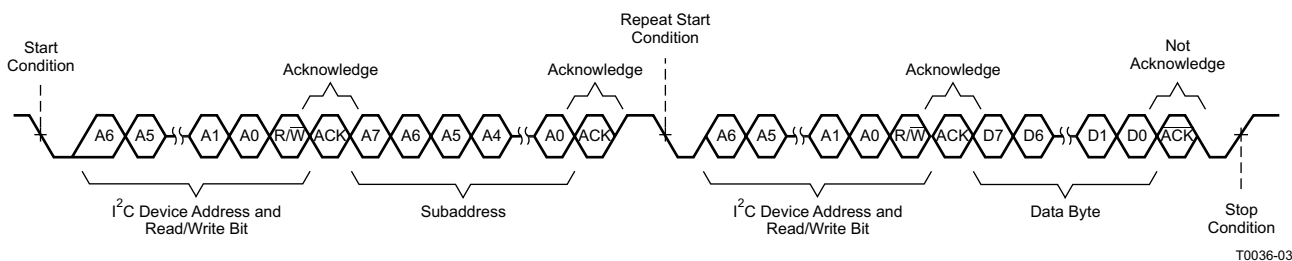
图 15. Random Read Transfer
