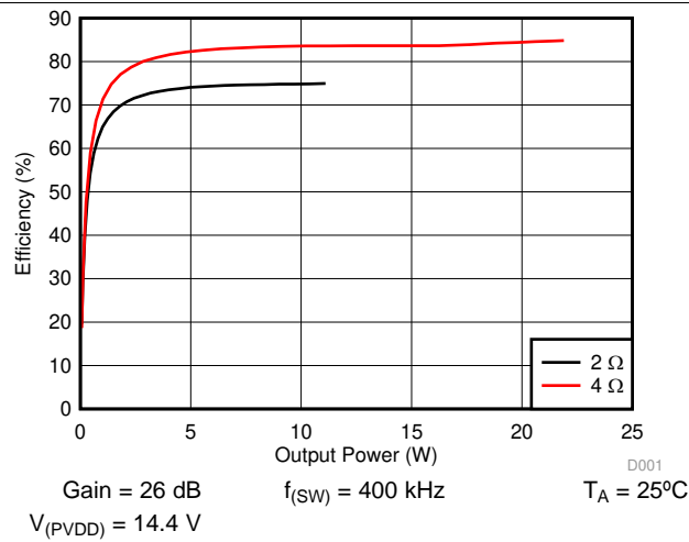
图 3. Efficiency vs Output Power
