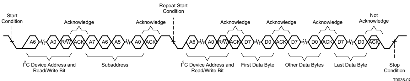
图 16. Sequential Read Transfer
