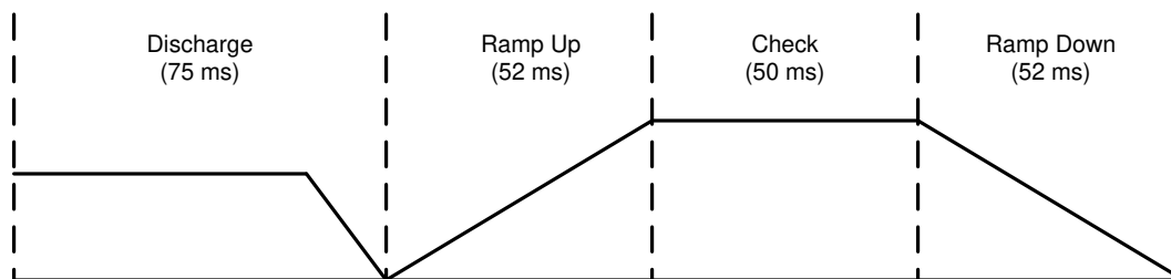
图 11. Load Diagnostics Sequence of Events
