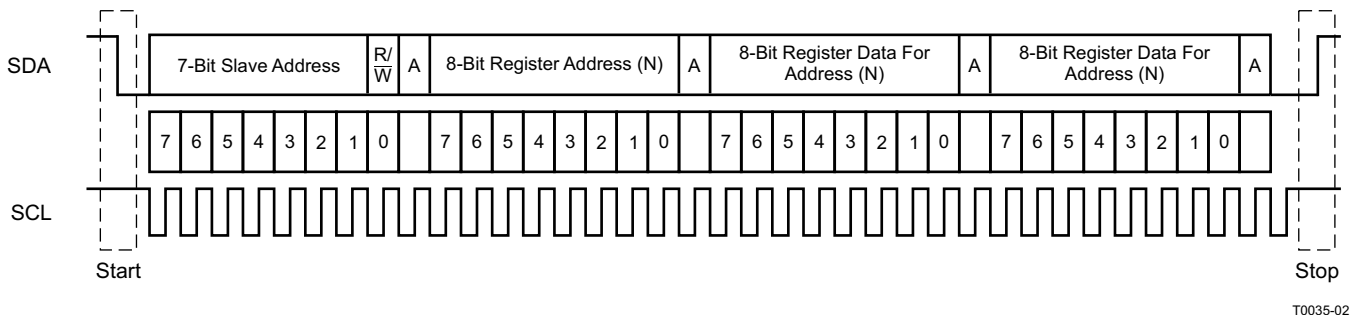
图 13. Typical I 2 C Sequence
