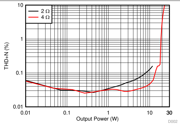
图 4. THD+N vs Output Power
