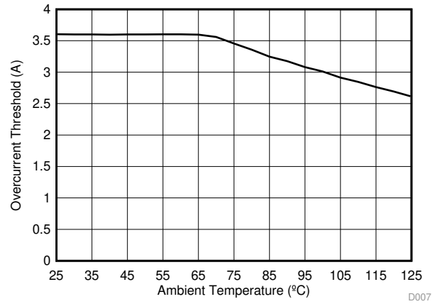
图 9. Overcurrent Threshold vs Temperature
