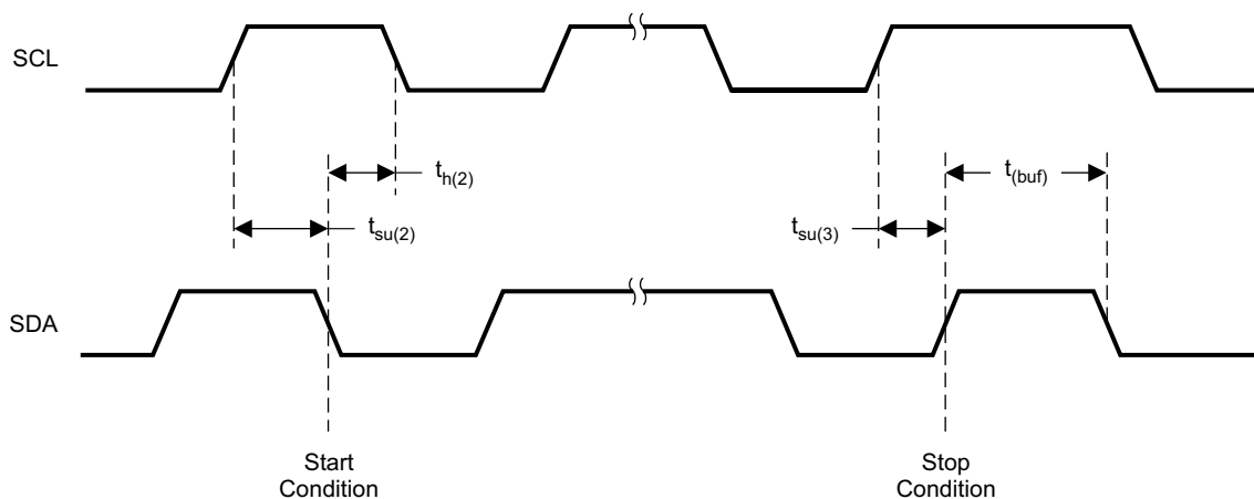
图 2. Timing for Start and Stop Conditions
