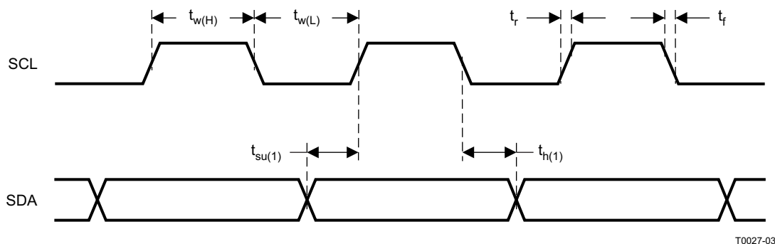
图 1. SCL and SDA Timing
