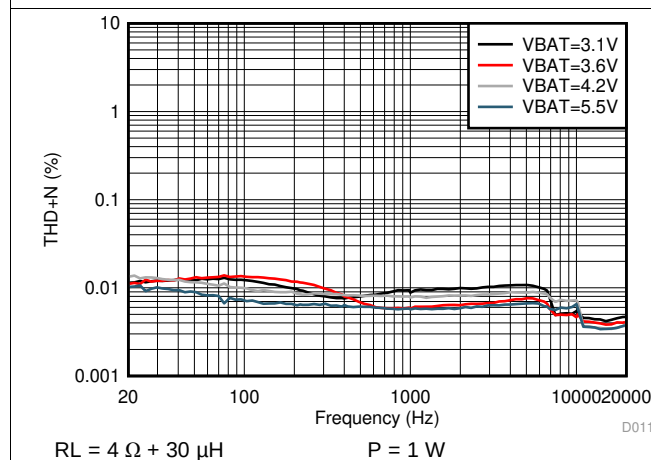
Figure 15. THD+N vs Frequency
