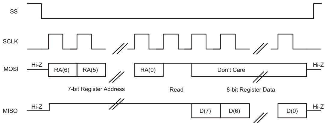
图 52. SPI Timing Diagram for Register Read
