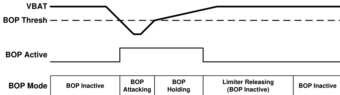
图 65. Brown Out Prevention Event
