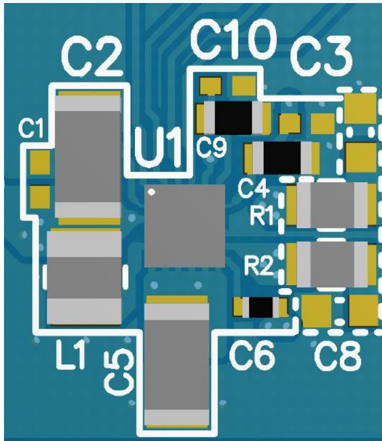
图 132. TAS2563 Board Layout
