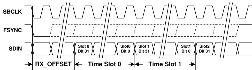
图 60. TDM RX Time Slots
