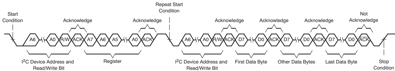
图 56. Multi-Byte Read Transfer
