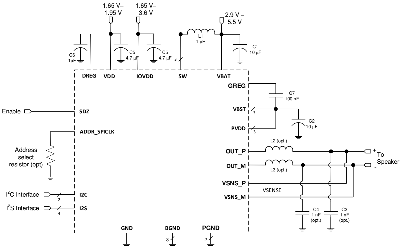
图 129. Typical Application - Digital Audio Input
