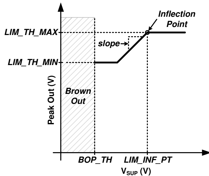
图 64. Limiter with Inflection Point and Minimum Threshold
