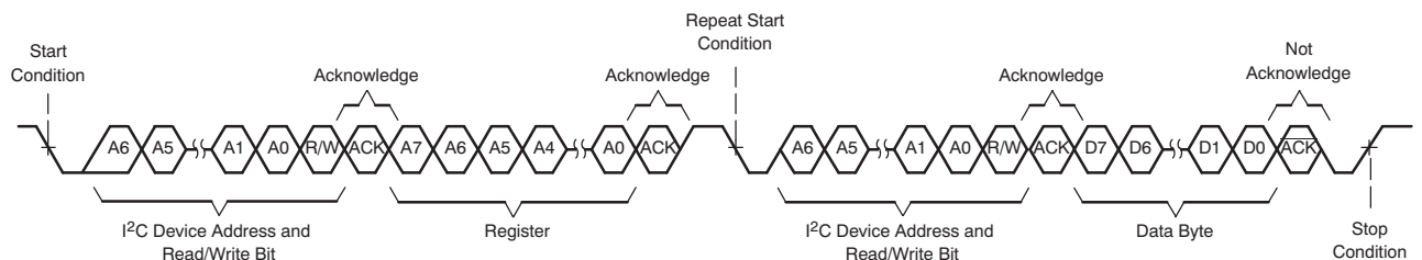
图 55. Single-Byte Read Transfer
