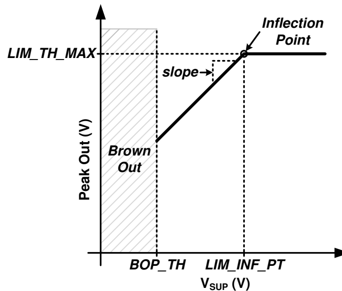
图 63. Limiter with Inflection Point
