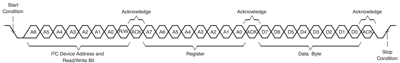
图 53. Single-Byte Write Transfer
