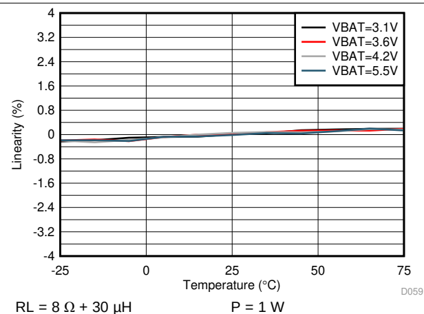
Figure 46. V-sense Linearity vs Temperature
