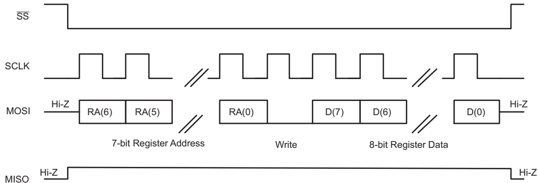
图 51. SPI Timing Diagram for Register Write
