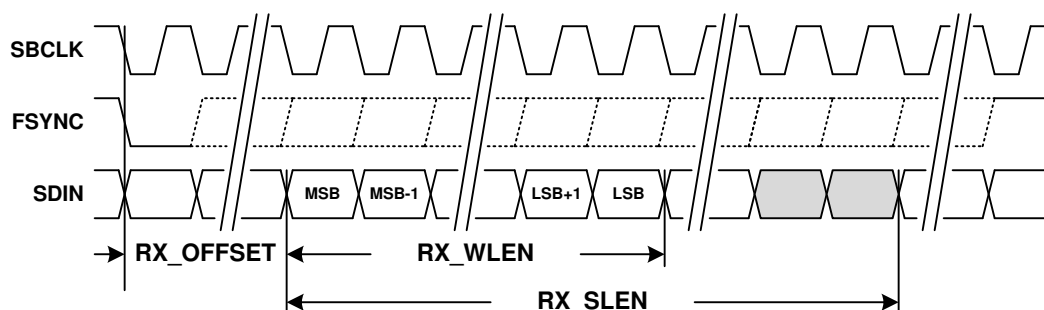
图 59. TDM RX Time Slot with Left Justification
