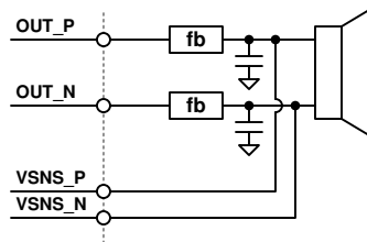
图 66. V-Sense Connections
