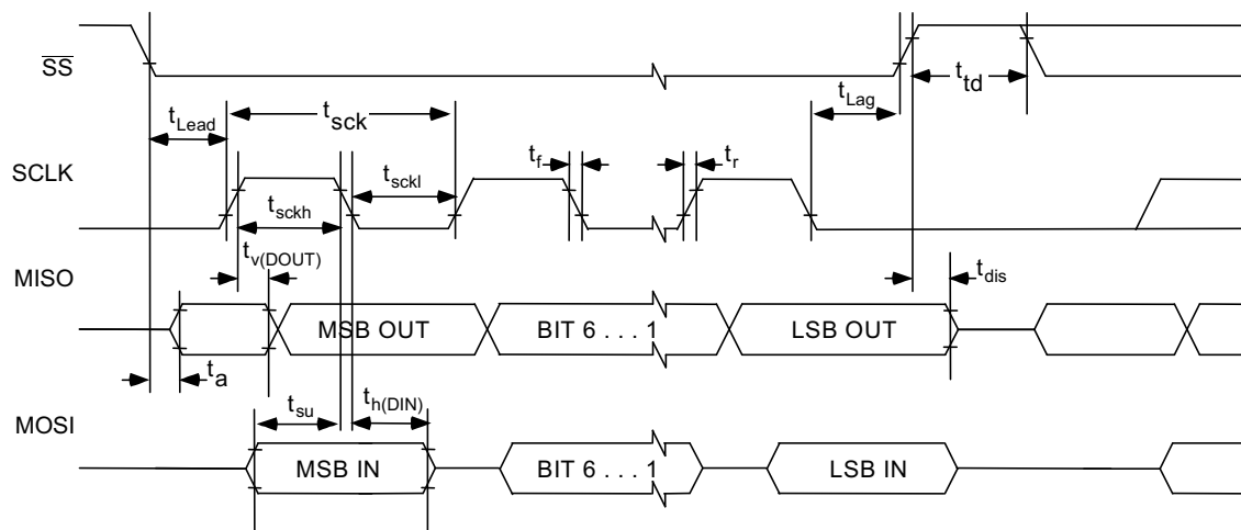
图 4. SPI Interface Timing Diagram
