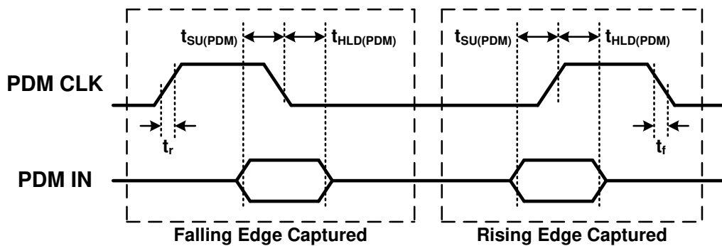
图 3. PDM Timing Diagram
