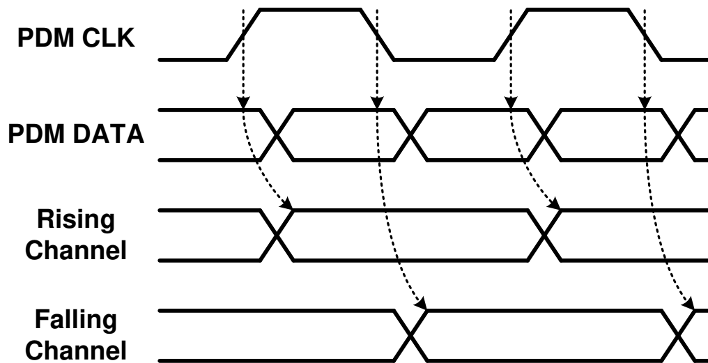
图 58. PDM Waveform
