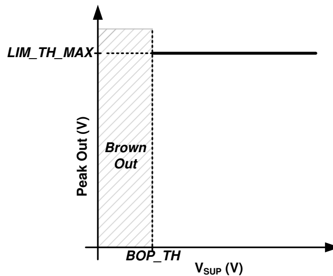
图 62. Limiter with Fixed Threshold
