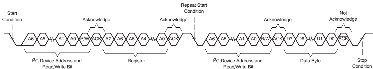
图 53. Single-Byte Read Transfer
