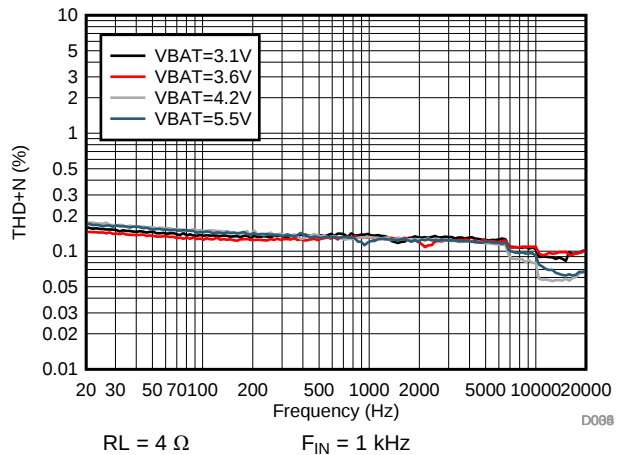
Figure 36. I-sense THD+N vs Frequency
