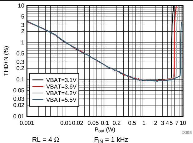
Figure 38. V-sense THD+N vs Output Power
