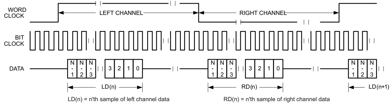
图 37. Timing Diagram for Left-Justified Mode with ASI_OFFSET1 = 1
