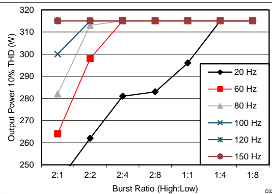
图 37. Maximum Burst Output Power vs Frequency, BTL, 4Ω Load, Each Channel, T_C = 75^\circ\text{C} , Power Ratio 1:8
