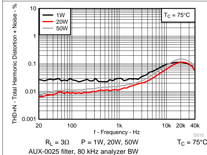
图 15. Total Harmonic Distortion+Noise vs Frequency
