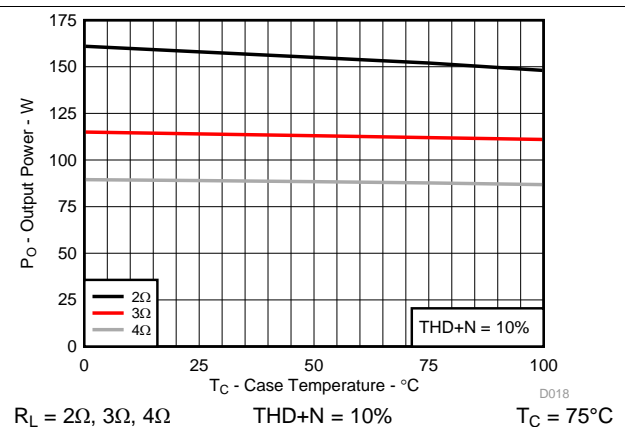
图 18. Output Power vs Case Temperature
